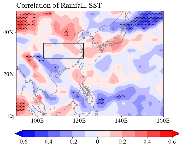
Fig. R1 Same as Fig. 2a, but for July.
