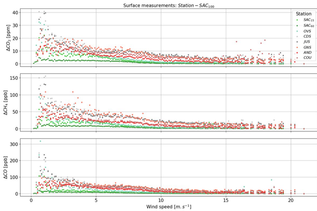
Figure S1 : \text{CO}_2 , \text{CH}_4 and \text{CO} gradients between stations and \text{SAC}_{100} (background) as a function of the wind speed ( \text{m}\cdot\text{s}^{-1} ), with 0.1 \text{ m}\cdot\text{s}^{-1} bins.
