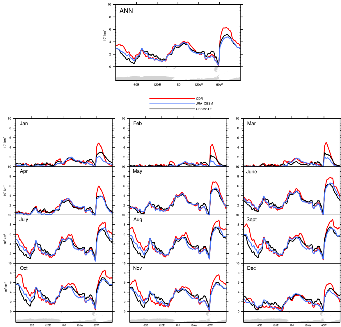
Figure S1. 1979-2020 Annual (top) and monthly (bottom panels) mean total sea ice extent as a function of longitude for the CDR (red), JRA-CESM (blue) and CESM2-LE data. Thick solid line indicates the mean (or ensemble mean for the CESM2-LE), shaded polygon indicates the mean \pm 1 standard deviation.
