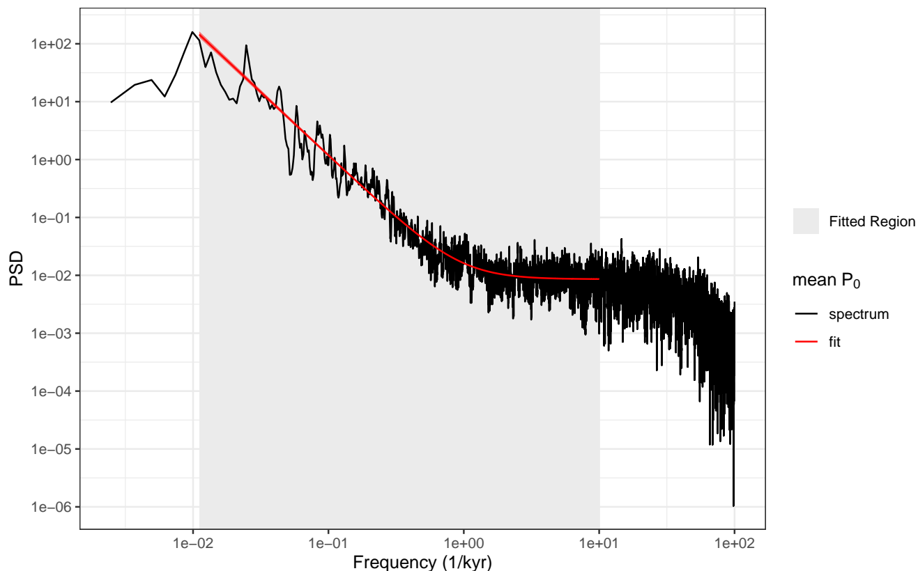
Figure 2. P_0 fit (red) over the grey shaded region of a composite power spectrum of the EDC water isotope record (black). By excluding high frequencies attenuated by firm diffusion, this fit serves as a good approximation of the initial isotopic variability of the BE-OIC
