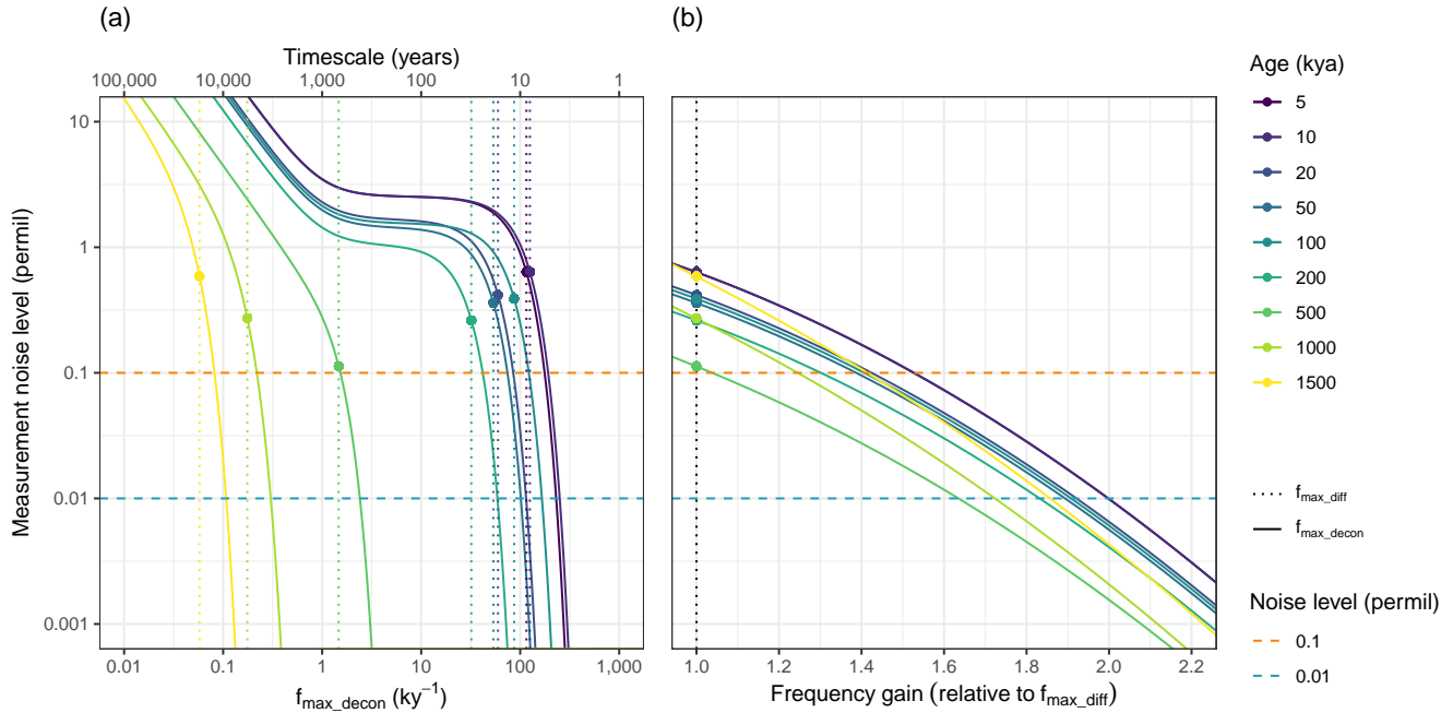
Figure 5. (a) Maximum permitted measurement noise to recover the highest resolvable frequency f_{\max\_decon} for selected ages of the BE-OIC after deconvolution, using A_{\min} = 0.25 . Also shown are the highest resolvable frequencies with no deconvolution f_{\max\_diff} (vertical dotted lines). For improved visibility, the points at which the f_{\max\_diff} lines intersect the corresponding f_{\max\_decon} lines are marked by dots. The horizontal dashed lines represent a typical measurement noise of 0.1‰ (orange) and a 10 times reduction (blue). (b) Same as (a) but showing the frequency gain relative to the corresponding f_{\max\_diff} (no deconvolution).
