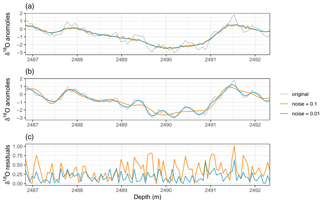
Figure 7. Example of the effect of the measurement noise level on the deconvolution in the depth domain for deep ice. (a) The true, undiffused record (grey) and two diffused records ( \sigma = 0.15 m) with measurement noise standard deviations of 0.1\text{‰} (orange) and 0.01\text{‰} (blue). (b) Deconvolutions of the two diffused records in (a). (c) Residuals between the original and deconvolved records.
