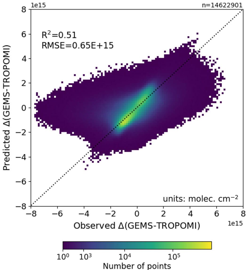
490 Figure 4: Predicted versus observed \Delta(\text{GEMS-TROPOMI}) in the test dataset. Colorscale shows density of points. The dashed line indicates the 1:1 line. R 2 and root mean square error (RMSE) are given inset.
