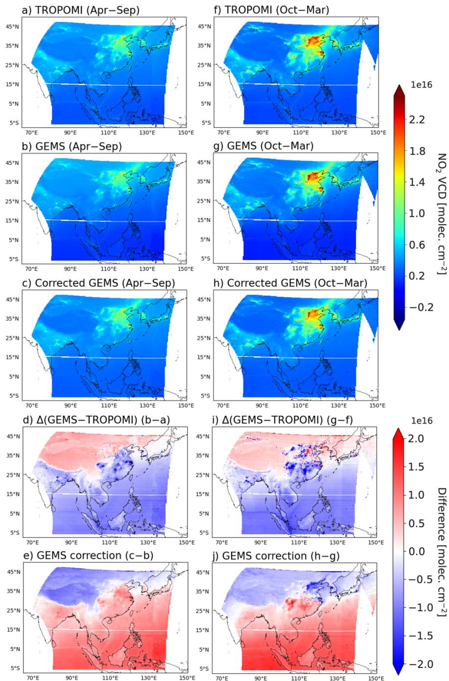
495 Figure 5: Comparison of TROPOMI, GEMS, and corrected GEMS \text{NO}_2 products in the GEMS scan domain. (a–c) \text{NO}_2 total VCDs averaged for April–September at the TROPOMI overpass time. The TROPOMI and GEMS data have been reprocessed to common GEOS-Chem vertical profiles for the observation scenes. (d) \Delta(\text{GEMS}-\text{TROPOMI}) for April–September. (e) Correction to the GEMS product for April–September. (f–j) Same as panels (a–e) but for October–March.
