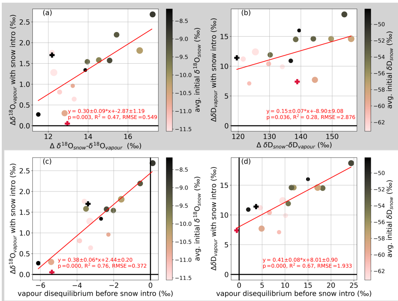
Figure S3 Change in vapour isotopic composition with snow introduction is better described assuming isotopic fractionation during sublimation
