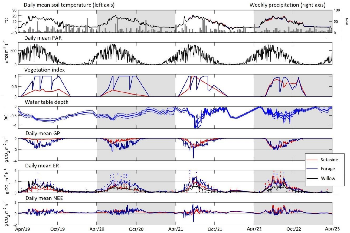
305 Figure 1: Daily mean of soil temperature and precipitation, photosynthetically active radiation (PAR), vegetation index, water table depth (site mean±std), gross photosynthesis, measured (dots) and model predicted (line) ecosystem respiration (soil respiration for willow) and net ecosystem exchange. Annual modelling periods (Apr - Mar) are marked with light grey or white background.
