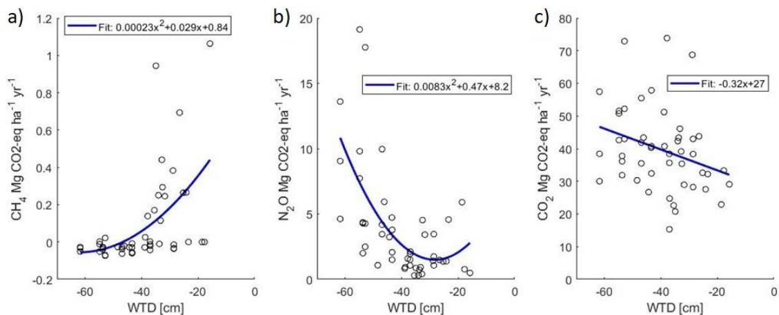
360 Fig. 2. Plot-wise mean annual fluxes of CH 4 (a), N 2 O (b) and soil respiration (c) (CO 2 eq.) as related to the mean annual WTD.
