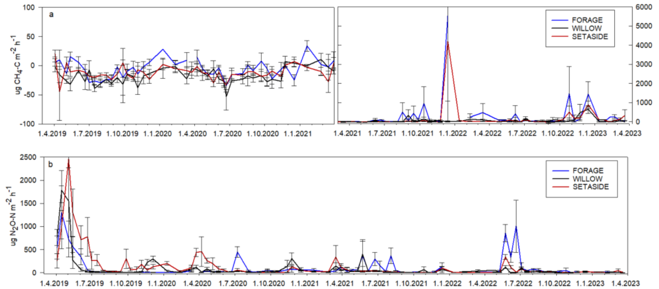
380 Fig. 3. Fluxes of CH 4 (a) and N 2 O (b) in 2019-2023. The error bars denote standard error. Note the different scale in the y- axis of (a) for the latter half of the period.
