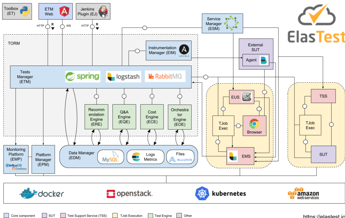
Figure 1: ElasTest Architecture
