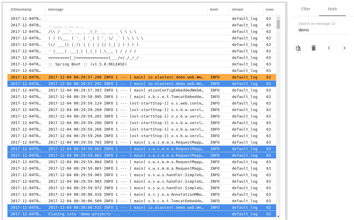
Figure 2: ElasTest Log Visualization
