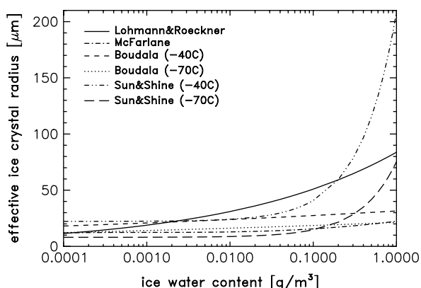
Figure 4. Different parametrizations of effective ice crystal radius as a function of ice water content. The parametrizations were taken from Lohmann and Roeckner (1996), McFarlane et al. (1992), Boudala et al. (2002), and Sun and Shine (1994). For those parametrizations that depend on temperature in addition to the ice water content, two different temperatures ( -40^\circ\text{C} and -70^\circ\text{C} ) were applied.
