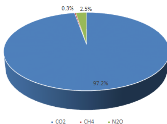
Figure 8-2 GHG Emissions by Gas in Macao in 2010
