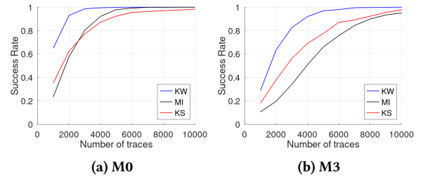
Figure 9: Attack modular addition with partition based distinguishers on M0 and M3 with 1000 repetitions
