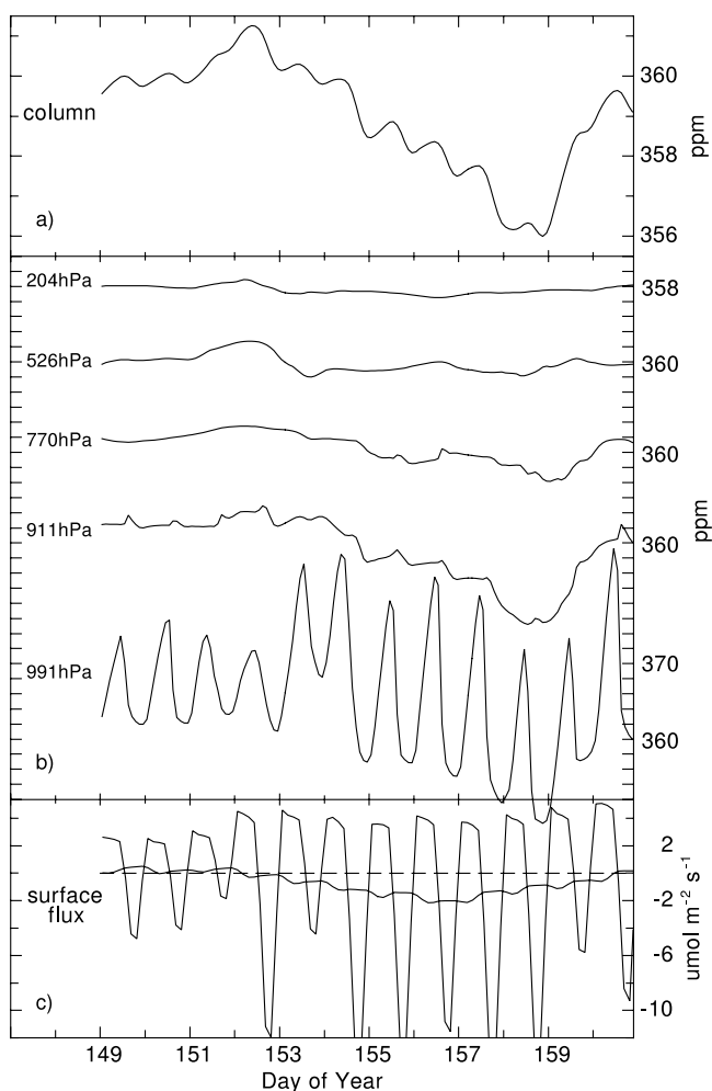
Figure 2. (a) Modeled column CO 2 , (b) CO 2 mixing ratios at 991, 911, 770, 526, and 204 hPa, and (c) diurnal and 5-day running mean surface CO 2 fluxes from the model grid cell containing the Park Falls/WLEF tower site for the period from 29 May (day 149) to 10 June (day 161).
