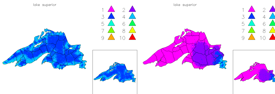
Figure 6.16: The mesh density for the global mesh (left) and for one of the local meshes (right) in the case N_P = 800K , P = 32 .
