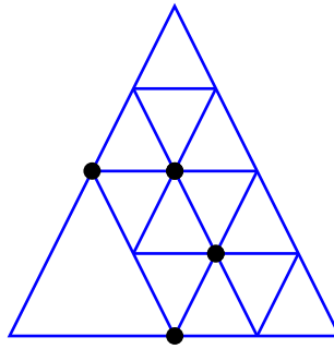
Figure 3.10: Four nonzero basis functions in t .
