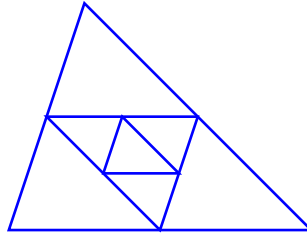
Figure 3.7: Non-conforming vertices created by red refinement.
