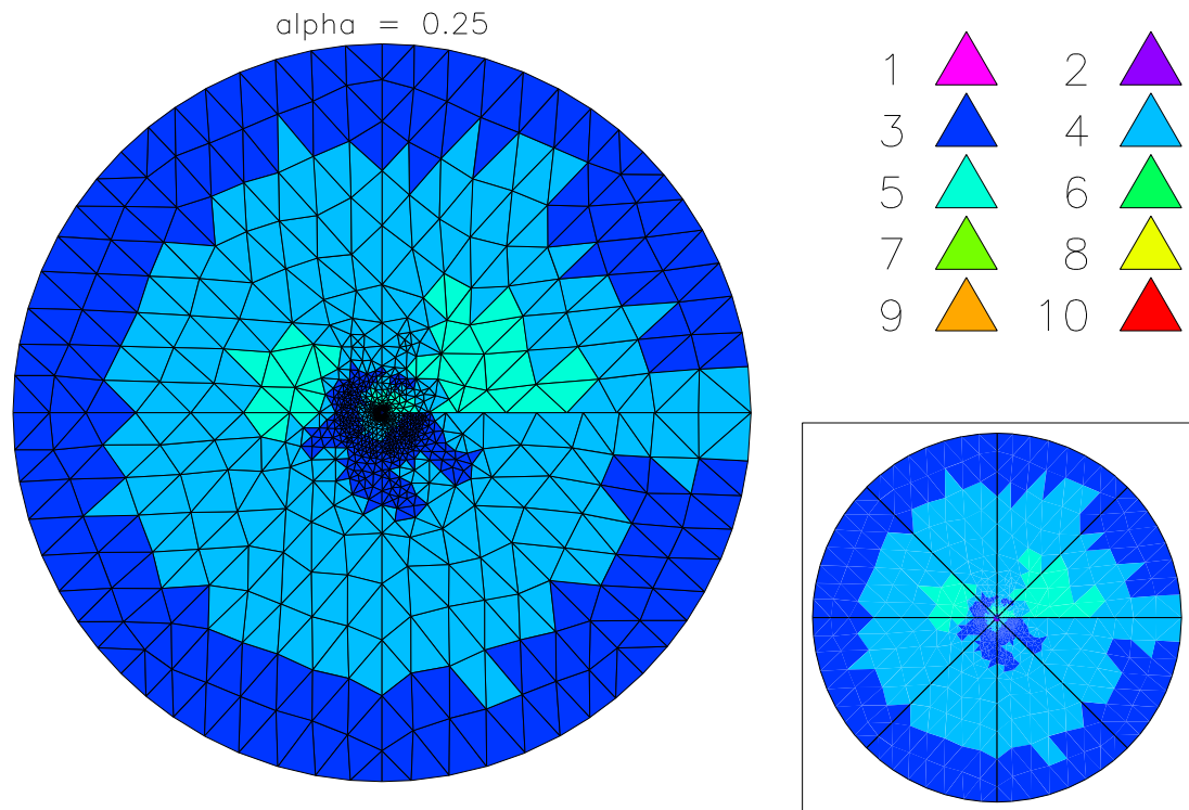
Figure 6.11: An adaptive mesh in automatic hp -adaptive ( N = 452220 )
