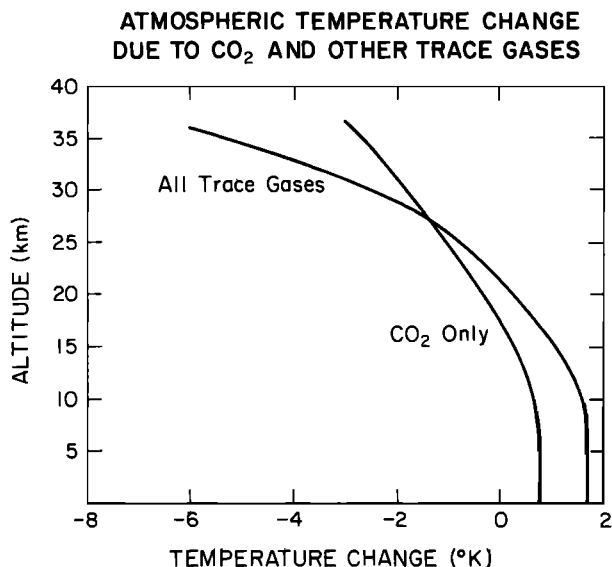
Fig. 4. Change in the vertical distribution of temperature due to an increase in CO 2 alone, and CO 2 along with all other trace gases listed in Figure 3. The trace gas increase scenario is as given by the "best estimate" values in Table 1a.
