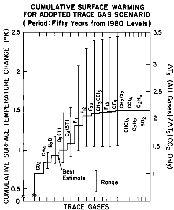
Fig. 3. Cumulative equilibrium surface temperature warming due to increase in CO 2 and other trace gases. Increases in gas amounts from 1980 values to 2030.
