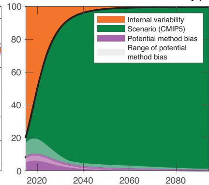
(b) Global annual decadal mean precipitation
