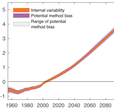
(b) Global annual decadal mean precipitation
