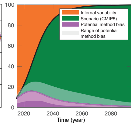
(b) Global annual decadal mean precipitation
