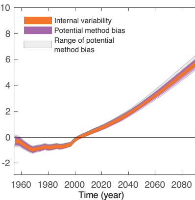
(b) Global annual decadal mean precipitation
