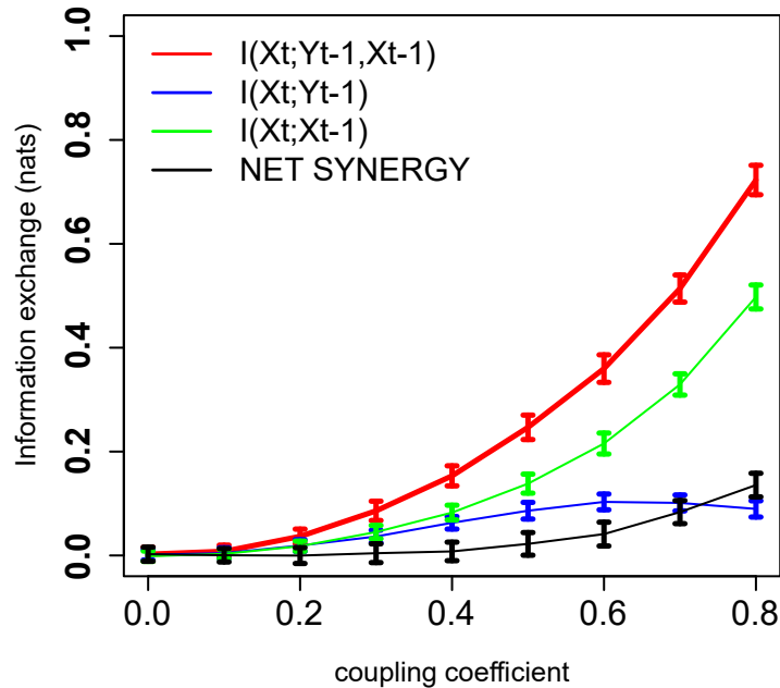
Kraskov
