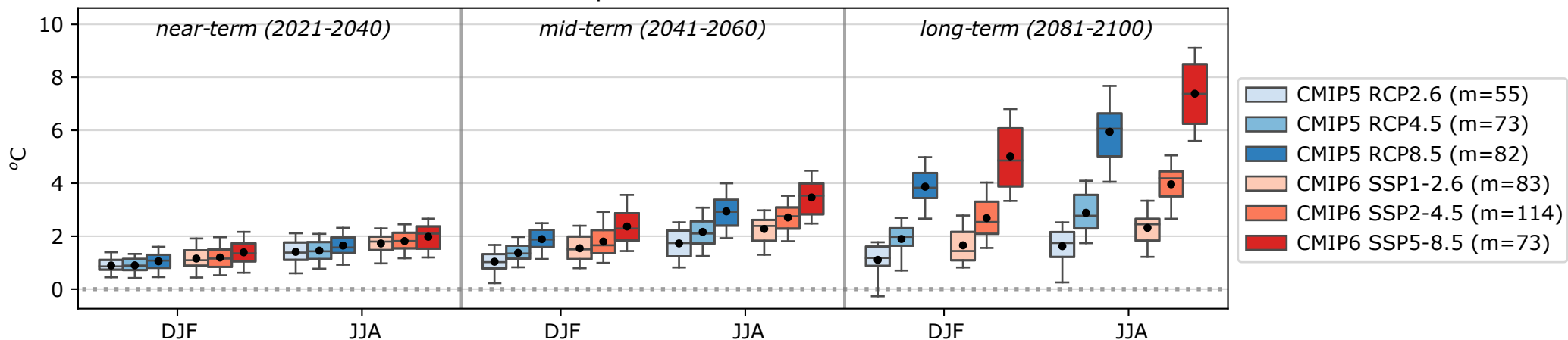
(a) Unweighted CMIP5 and CMIP6 TAS changes over JJA and DJF Baseline period: 1986-2005
