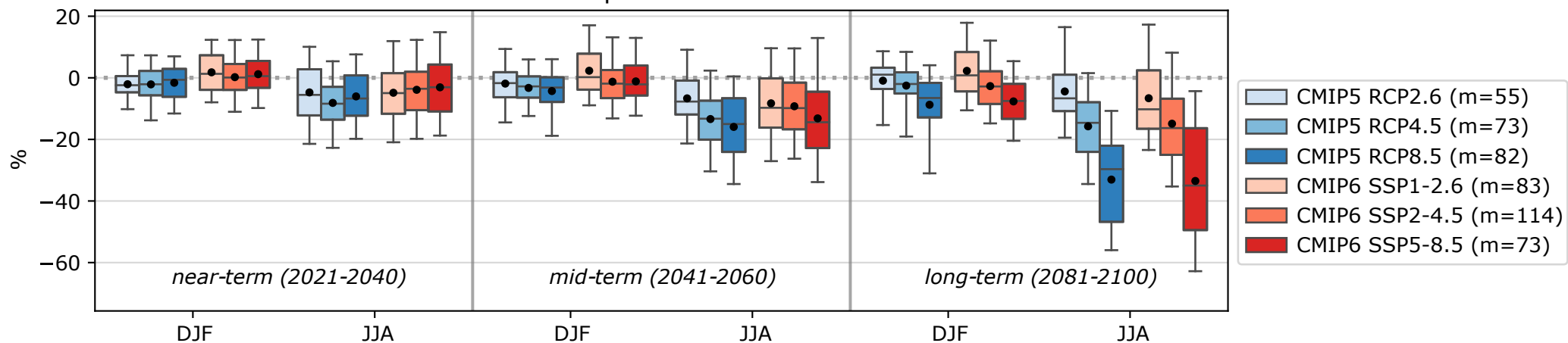
(c) Unweighted CMIP5 and CMIP6 PR changes over JJA and DJF Baseline period: 1986-2005
