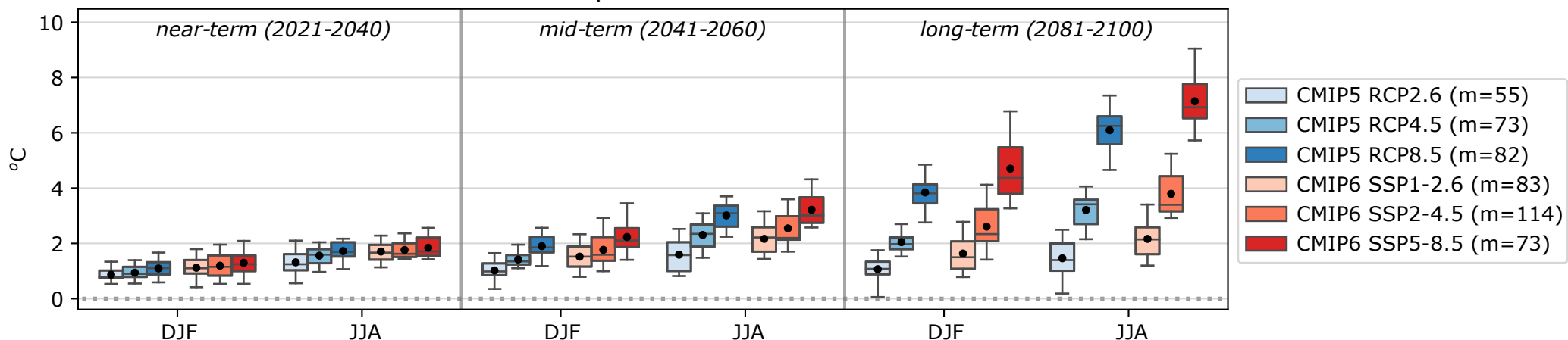
(b) Weighted CMIP5 and CMIP6 TAS changes over JJA and DJF Baseline period: 1986-2005
