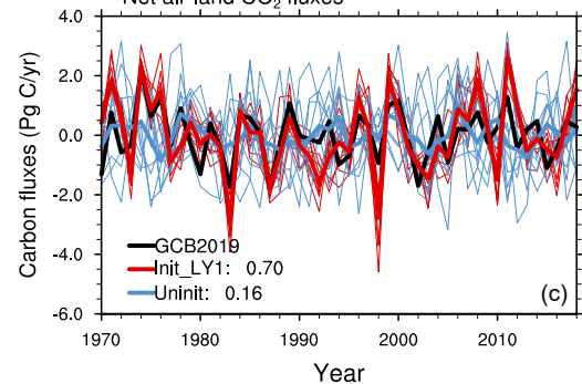
Net air-land CO 2 fluxes
