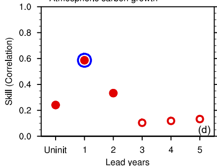
Atmospheric carbon growth
