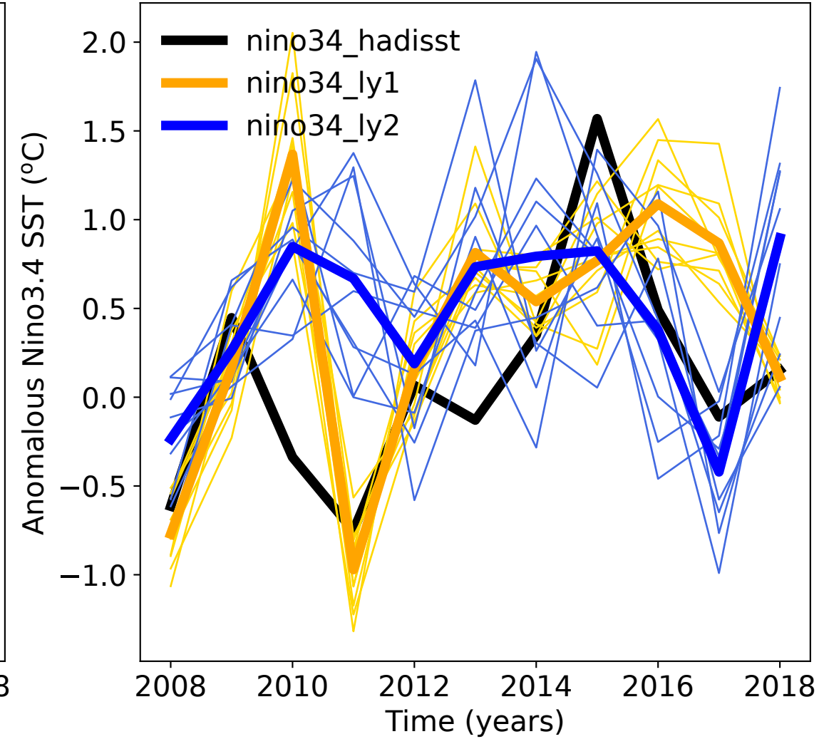
(c) Nino3.4 SST
