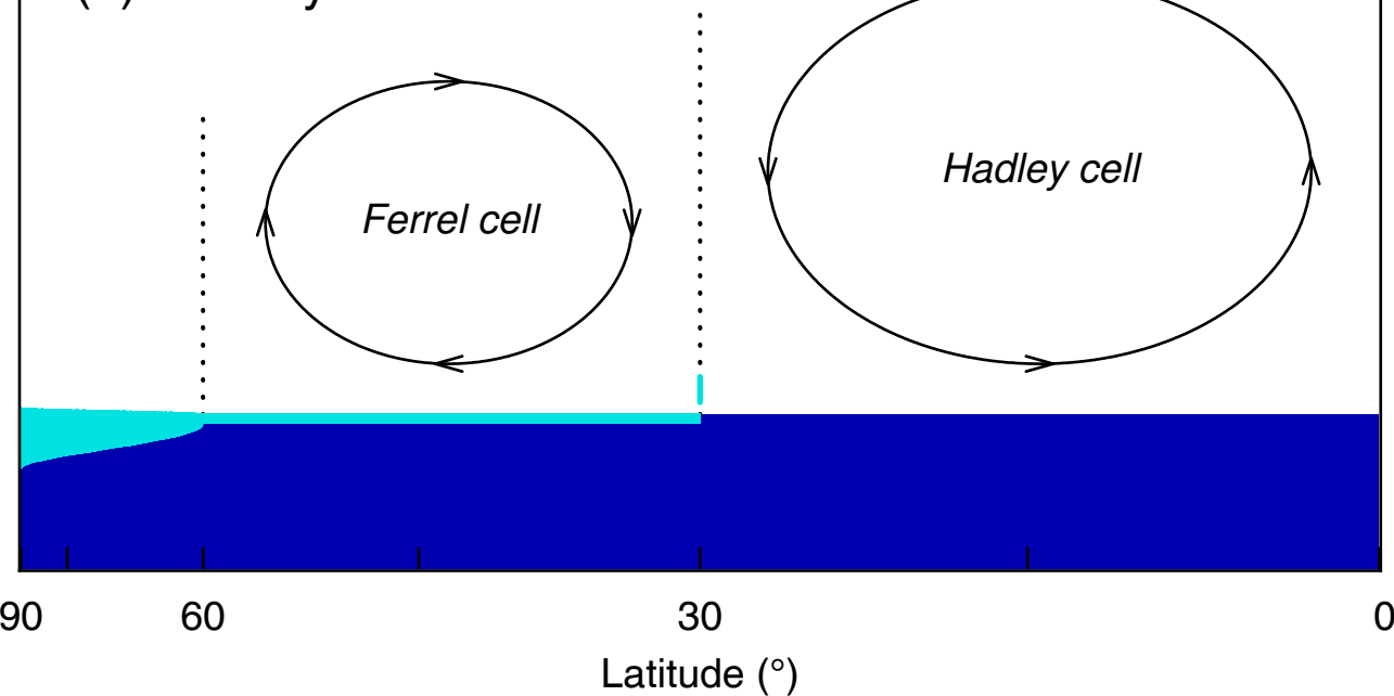
(b) Hadley state
