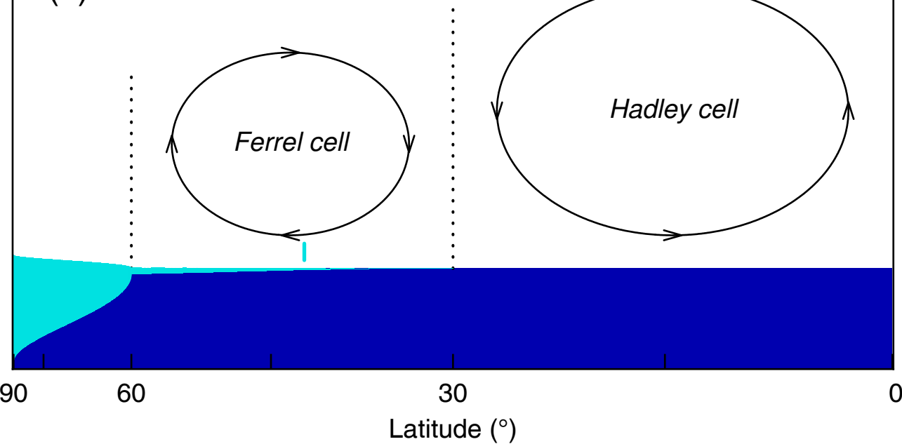
(a) Ferrel state
