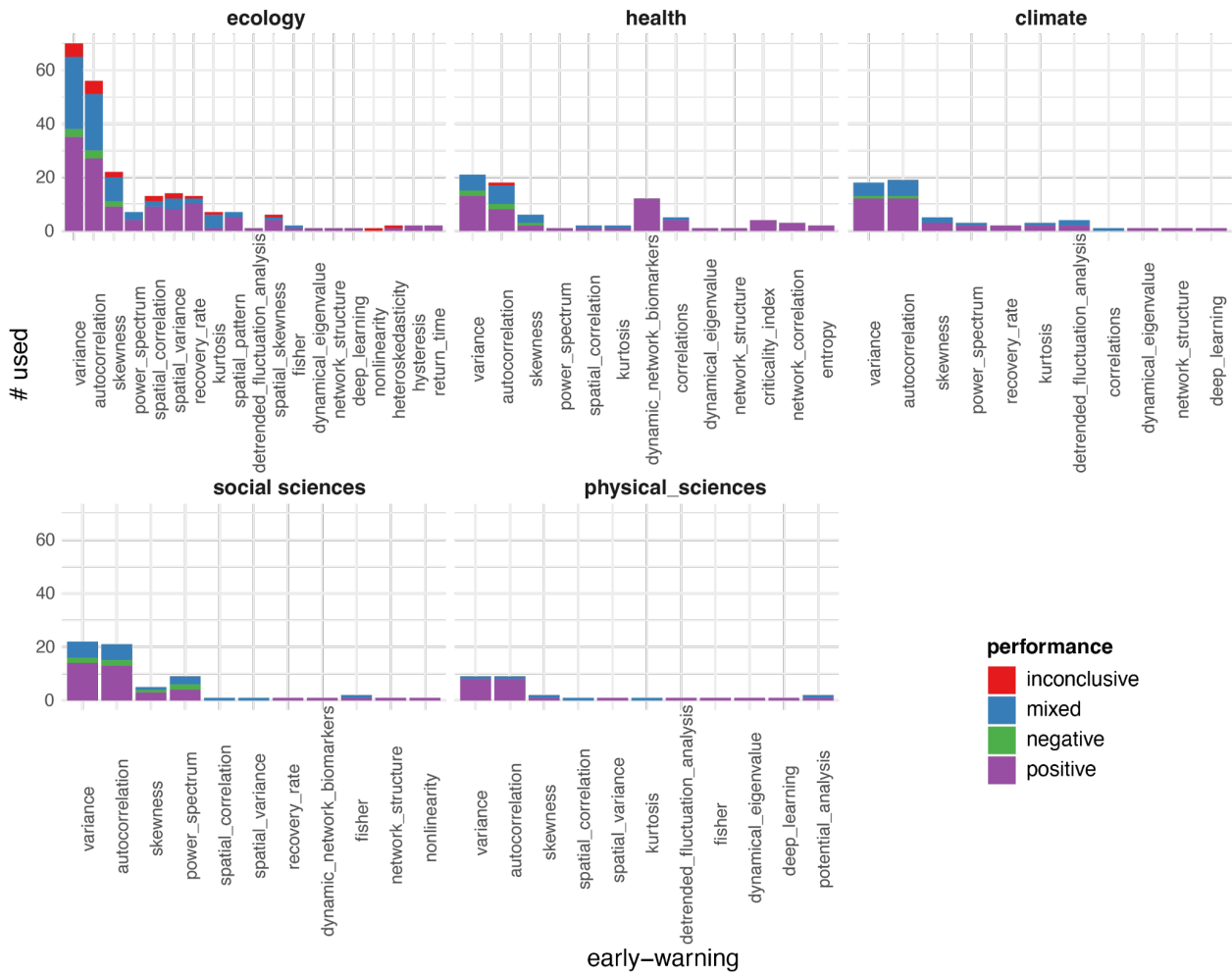
Figure S5: Performance of early-warnings used more than once per domain
