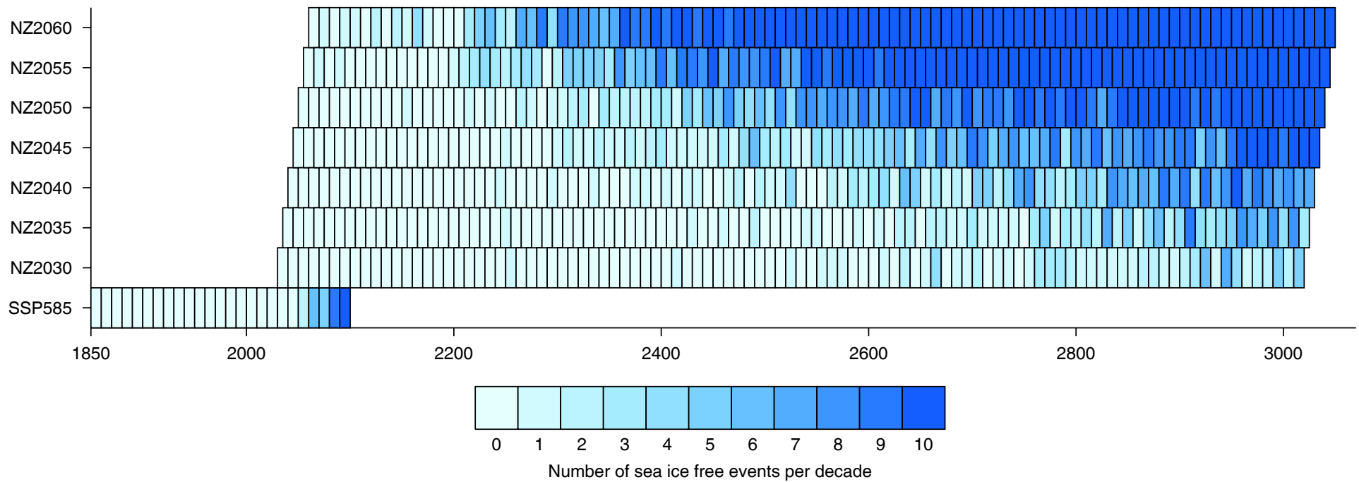
(b) Antarctic sea ice free Marchs
