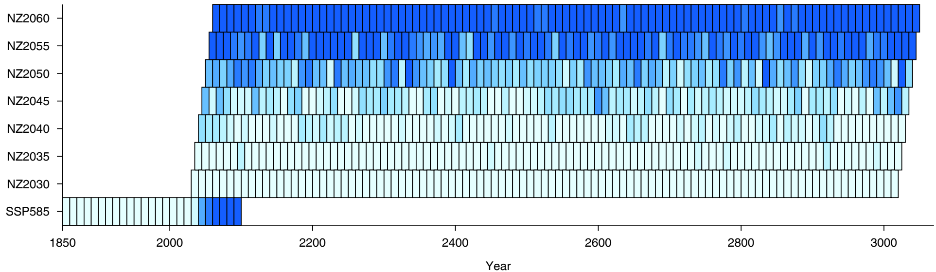
(b) Antarctic sea ice free Marchs
