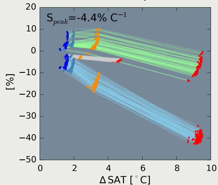
(a) Change in oceanic O 2 inventory
