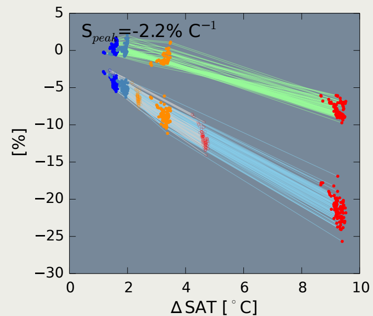
(c) Change in POM export (30° S–30° N)
