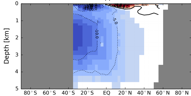
(g) Indo-Pacific meridional overturning [Sv] PI
