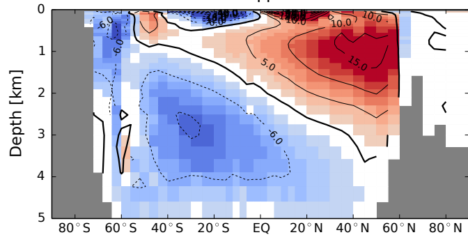
(a) Meridional overturning circulation [Sv] PI
