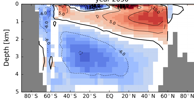
(b) Meridional overturning circulation [Sv] year 2050
