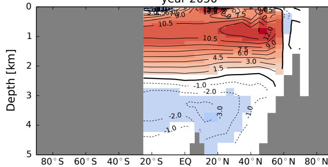
(e) Atlantic meridional overturning [Sv] year 2050
