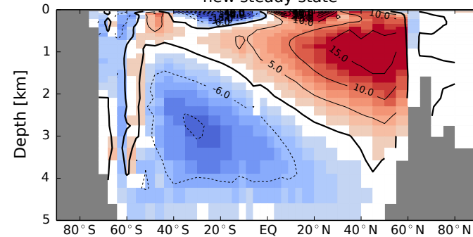
(c) Meridional overturning circulation [Sv] new steady state
