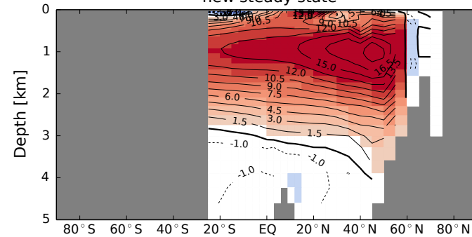
(f) Atlantic meridional overturning [Sv] new steady state
