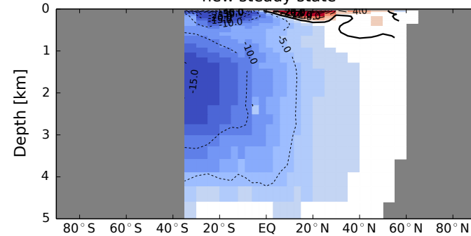
(i) Indo-Pacific meridional overturning [Sv] new steady state
