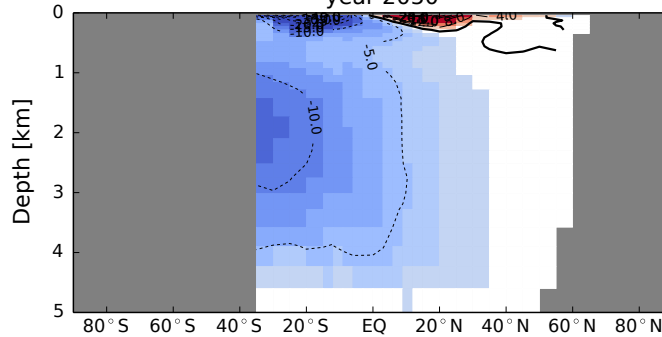
(h) Indo-Pacific meridional overturning [Sv] year 2050
