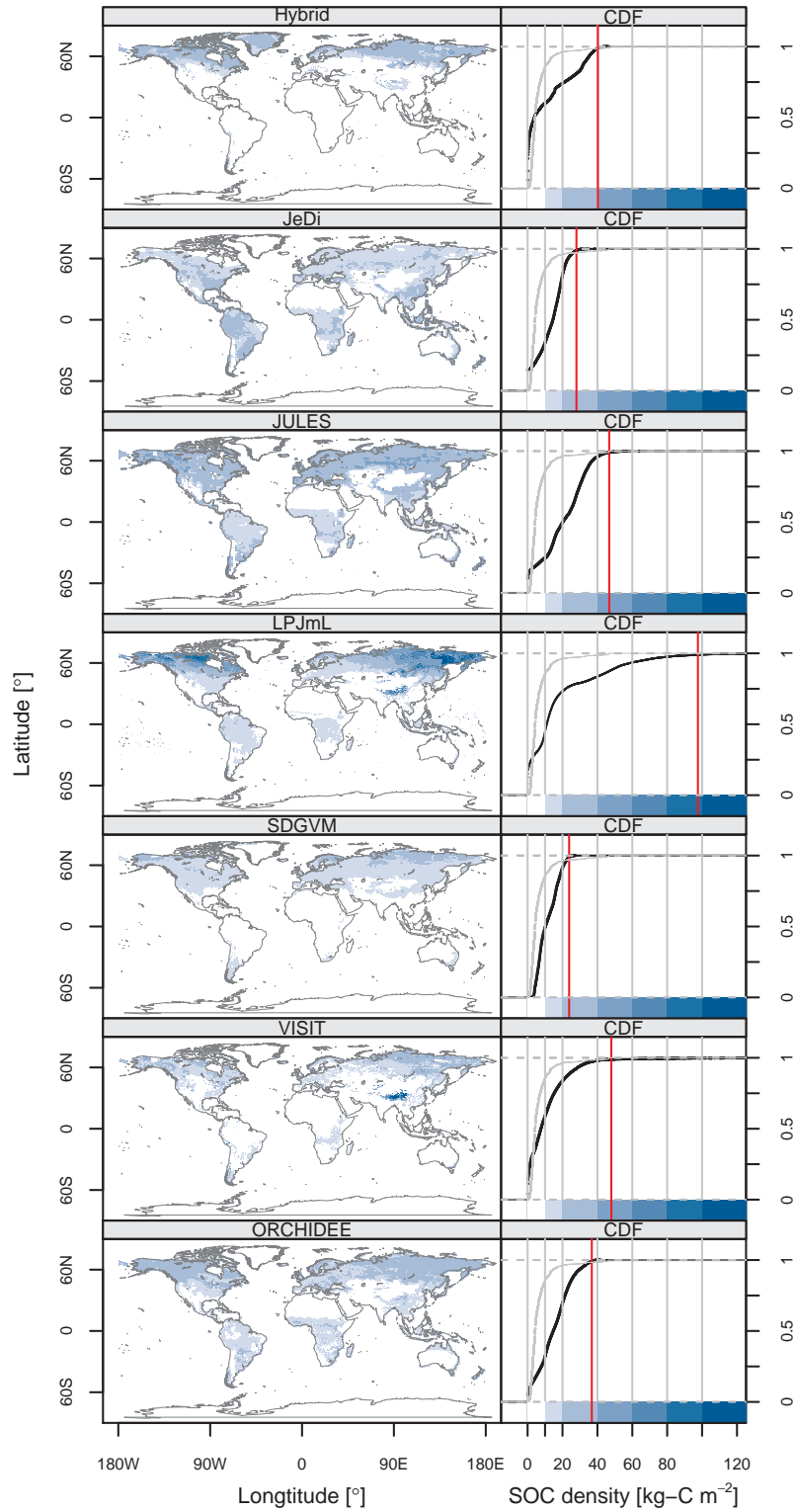
FIGURE 15. Maps of SOC density in 2000 and CDF in each biome model with HadGEM RCP8.5. In CDFs, red line indicates the 99th percentile of SOC density. In each CDF, grey lines indicate the CDF from the SOC density from the original Harmonized World Soil Database.
