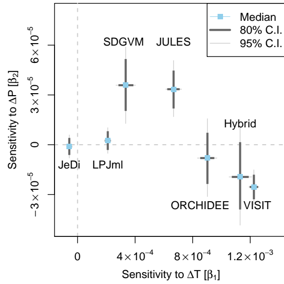
FIGURE 3S. Sensitivity of global SOC stocks in response to \Delta T and \Delta P in each biome model
