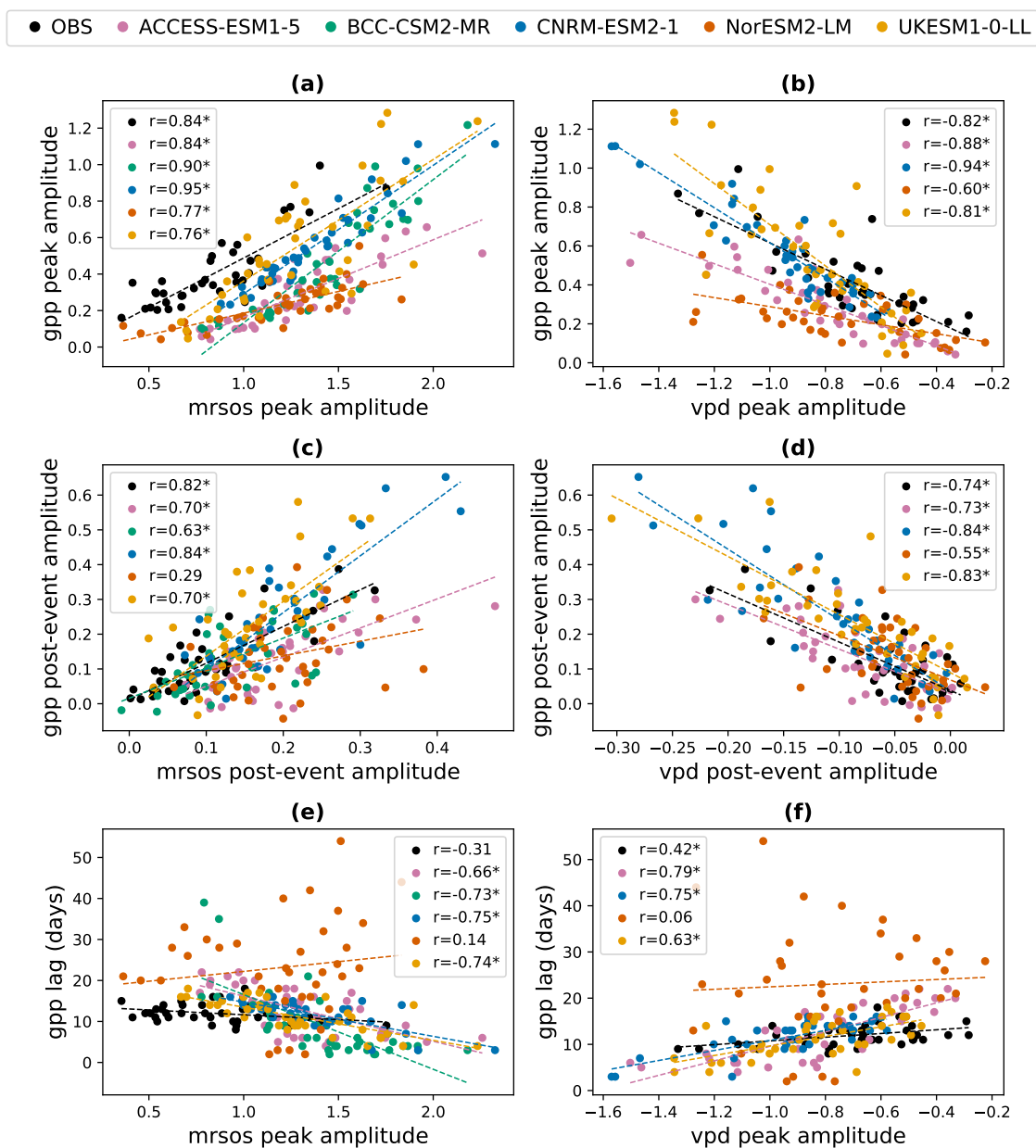
Figure 4. Regional GPP responses to intraseasonal wet events compared to the driving perturbations in surface soil moisture (a, c, e) and vapour pressure deficit (b, d, f). Each scatter point represents an IPCC AR6 region. Dashed lines show linear best fits. The legend for each panel indicates the linear correlation coefficient between the driving perturbation and the GPP response for each model. Asterisks after correlation coefficients denote significance at the 95% level. The uppermost legend, showing which model is denoted by each colour, applies to all panels. The observational products used are FLUXCOM-CRUJRAv1 (GPP), ESA CCI (surface soil moisture) and ERA5 (VPD).
