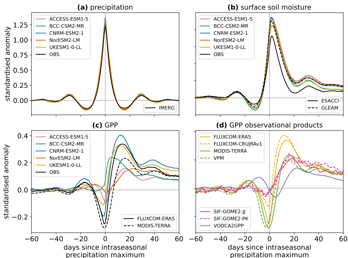
Figure 1. Composites of (a) precipitation (b) surface soil moisture and (c, d) GPP around intraseasonal wet events. All land pixels between 60°S and 80°N are included, except in months where the ground is frozen or in regions without valid ESA CCI soil moisture observations. The surface soil moisture and GPP composites have been scaled by the maximum amplitude of their corresponding precipitation composite.
