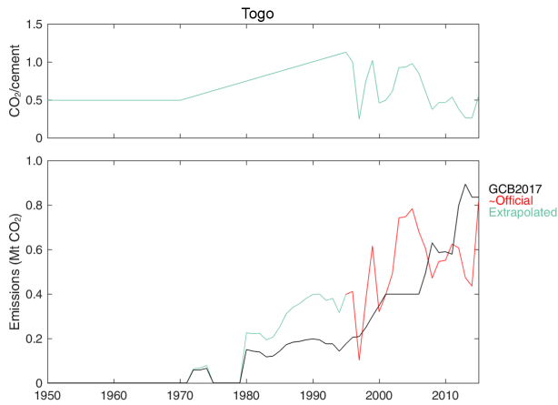
Figure C36. Revised cement emissions in Togo.
