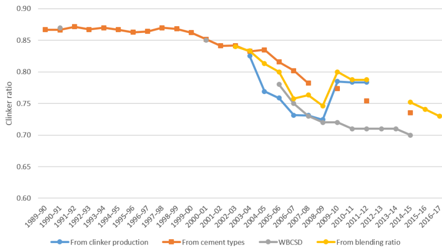
Figure C5. Estimates of clinker ratio in India from various sources.
