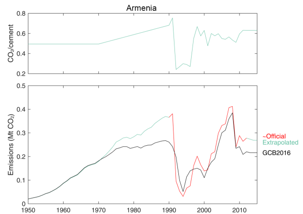
Figure C9. Revised cement emissions for Armenia.
