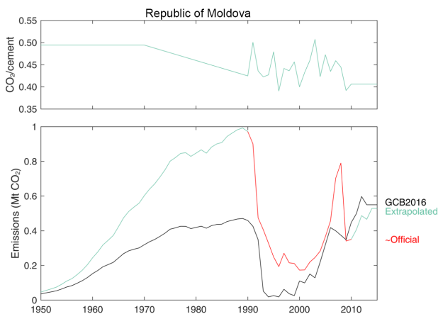
Figure C27. Revised cement emissions for Moldova.
