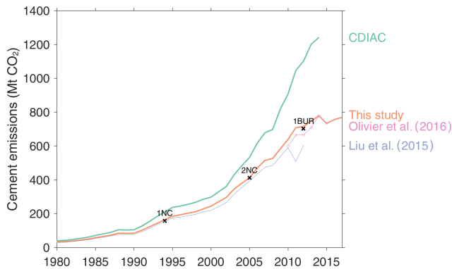
Figure 3. Process emissions from Chinese cement production, 1980–2017. 1NC refers to China’s first National Communication, 2NC the second National Communication, and 1BUR the first Biennial Update Report. Also shown are estimates from CDIAC (Boden et al., 2017), Liu et al. (2015) and EDGAR v4.3.2 FT2015.
