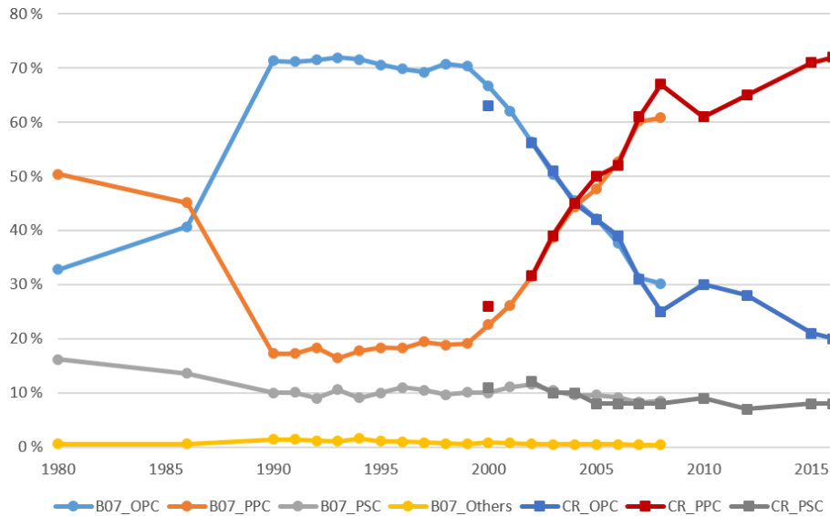
Figure C4. Proportions of cement production by type. B07: Bapata et al. (2007), CR: CRISIL ( https://www.crisil.com/ , last access: 31 March 2017). OPC: ordinary Portland cement, PPC: Portland pozzolana cement, PSC: Portland slag cement.
