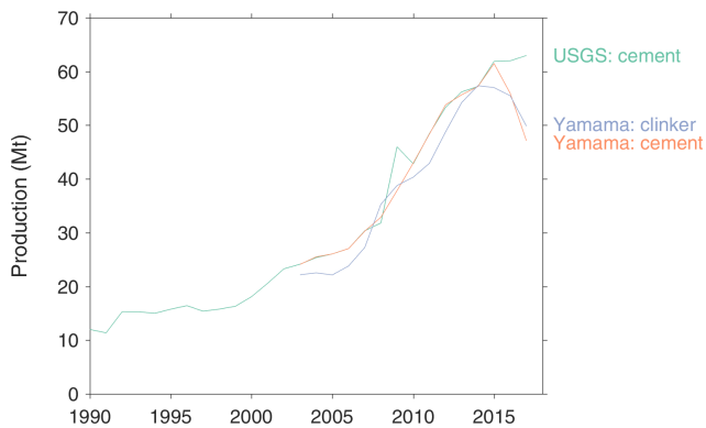
Figure C32. Saudi Arabian cement and clinker production, 1990–2017 (Yamama Cement, 2018; USGS, 2018; van Oss, 1994–2018).
