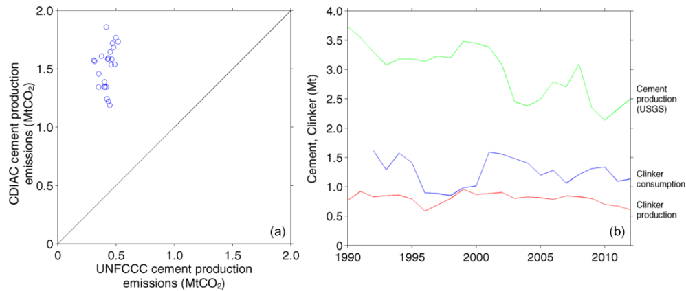
Figure A3. The Netherlands: (a) CDIAC vs. UNFCCC; (b) linker, cement. Note “Clinker consumption” is production plus imports less exports, but excludes stock changes. Sources: UNSD (2015), UNFCCC (2014), van Oss (1994–2018), and Boden et al. (2013).
