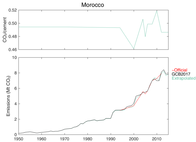
Figure C30. Revised cement emissions for Morocco.
