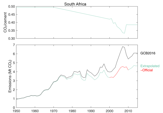
Figure C35. Revised cement emissions for South Africa.
