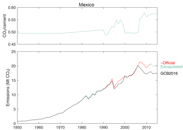
Figure C26. Revised cement emissions for Mexico.
