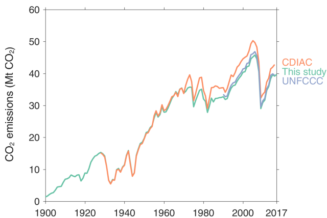
Figure C8. Revised cement emissions for USA.
