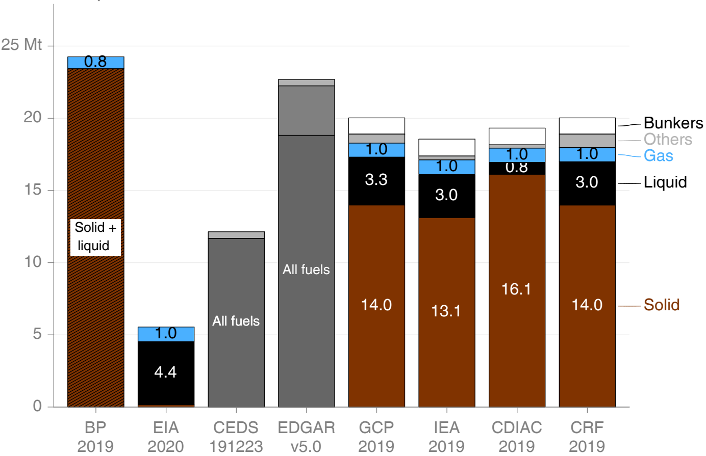
Comparison of fossil CO 2 emissions: Estonia 2014
