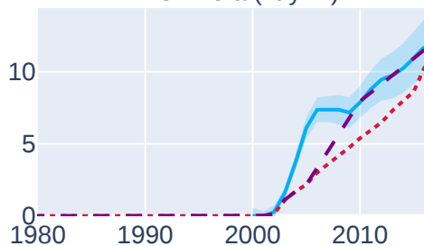
HFC-43-10-mee (kt yr -1 )
