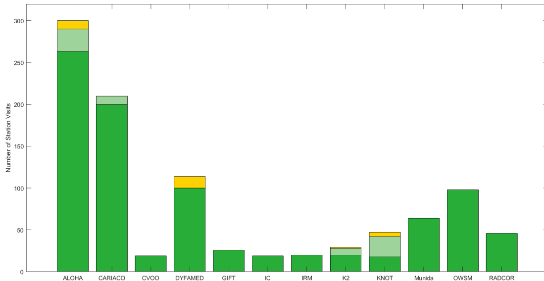
Figure 5. Assigned SOP flags per station exemplarily shown for TA. Flags have been assigned on a cruise-per-cruise basis, i.e., per station visit. The color scheme used is identical to that in Fig. 3.
