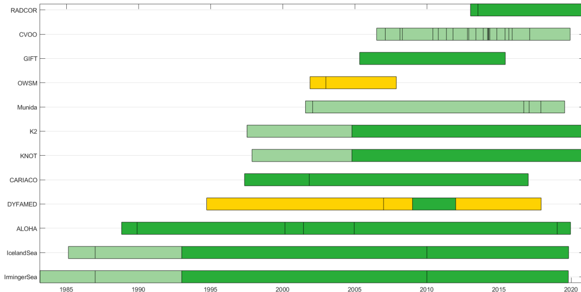
Figure 4. Time dependency of assigned SOP flag of each time-series program exemplarily shown for nitrate. Vertical black lines indicate method changes both captured and not captured (e.g., instrument change) by the SOP flags. The color scheme used is identical to that in Fig. 3. Note that DYFAMED changed back to poisoning the samples for conservation based on internal analyses of conservation methods.
