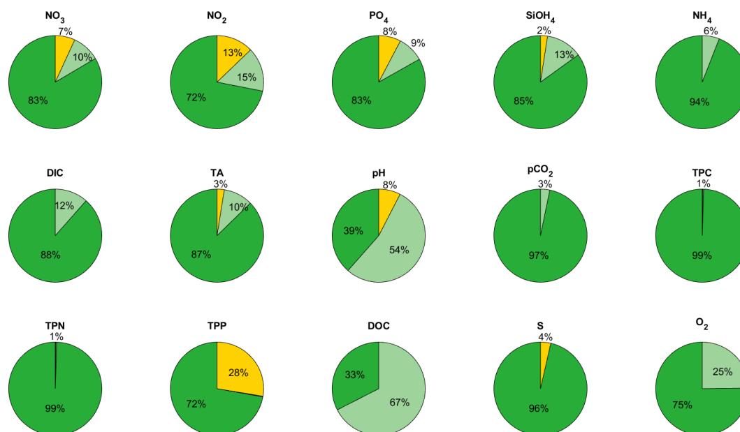
Figure 3. Overview of assigned SOP flags. Percentages correspond to the number of samples in the combined dataset. Dark-green colors indicate samples that have been measured according to all (including desired) SOP requirements, i.e., a SOP flag 1 (Table 2). Light-green colors indicate samples that have been measured meeting the required SOP requirements only, i.e., a SOP flag 2. Orange colors indicate samples for which the methods do not meet the SOP requirements, i.e., a SOP flag 3. Variable synonyms correspond to the product header names (Table 1). Note that total particulate matter includes the exclusively organic particulate matter measurements from CVOO.
