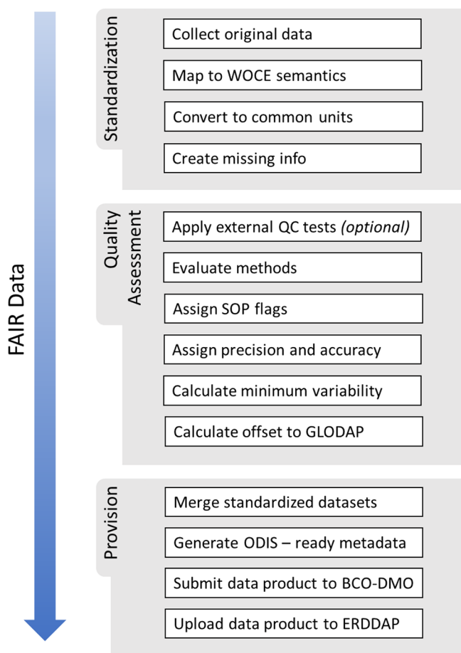
Figure 2. Schematic data flow of the SPOTS pilot.
