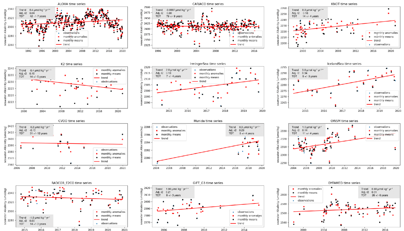
Figure 7. Trend analysis of TA in the mixed layer using TOATS. Data symbols show the original time-series observations (blue circles), the time series of monthly means (black circles), the de-seasoned monthly means (red squares), and the trend of the de-seasoned monthly means (red line) (From Sutton et al., 2022). The monthly anomalies (red squares) that are used for the trend analyses are shown as de-seasoned monthly means. The gray boxes include the yearly trend, adjusted R^2 , and the minimum trend detection time (TDT). An asterisk next to the yearly trend number indicates that the result is significant (two-sided t -test p value < 0.05 ). Note that the x and y axes are not in sync among the different time-series subplots.
