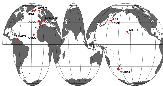
Figure 1. Locations of participating ship-based time-series stations.
