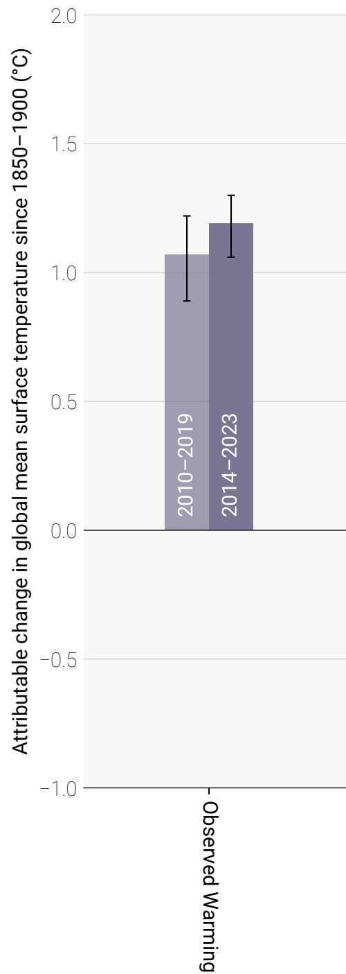
(a) Decade-average warming given by observations
