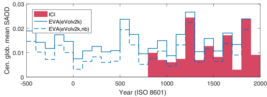
Figure 7. Centennial global mean SAOD from the ICI and EVA(eVolV2k) reconstructions. A version of the EVA reconstruction which includes no background sulfur injection, EVA(eVolV2k, nb), is shown by the dashed line.
