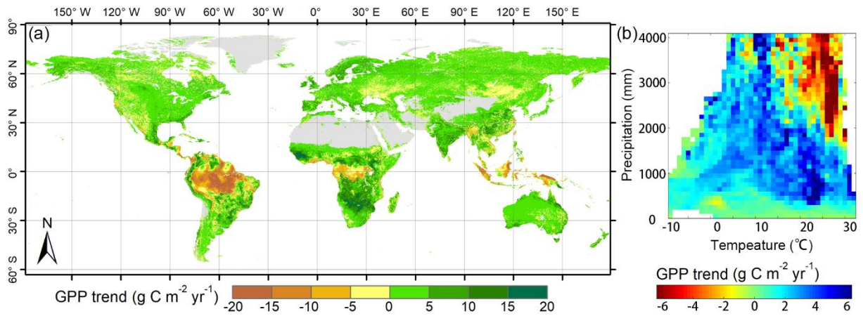
815 Figure 5b: Spatial pattern of global GPP trend simulated by the revised EC-LUE models during 1982–2017: (a) trend of annual GPP, (b) trend of annual GPP at different temperature and precipitation gradients.
