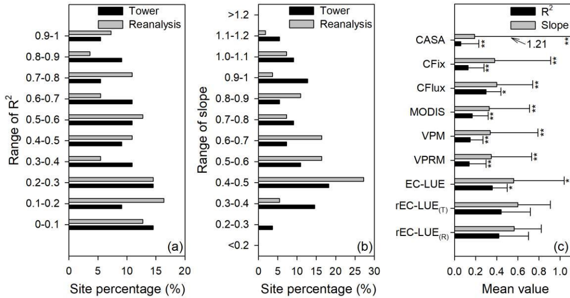
795 Figure 3: Site percentage of (a) correlation coefficients ( R^2 ), and (b) regression slopes between the model simulated and tower-based interannual variabilities in GPP. (c) Averaged values (error bars represent the standard deviations) of R^2 and slope for various LUE models. rEC-LUE (T) and rEC-LUE (R) indicate the revised EC-LUE models derived from tower-derived meteorology data and meteorological reanalysis dataset. The R^2 and slopes of the other seven LUE models (i.e., EC-LUE, VPRM, VPM, MODIS, CFlux, CFix, and CASA) in the figure were obtained from the study by Yuan et al. (2014). ** and * indicate a significant difference in statistic variables ( R^2 and slope) between the rEC-LUE (T) and other LUE models (i.e., rEC-LUE (T) and other seven LUE models) at p -value < 0.01 and p -value < 0.05, respectively. 800
