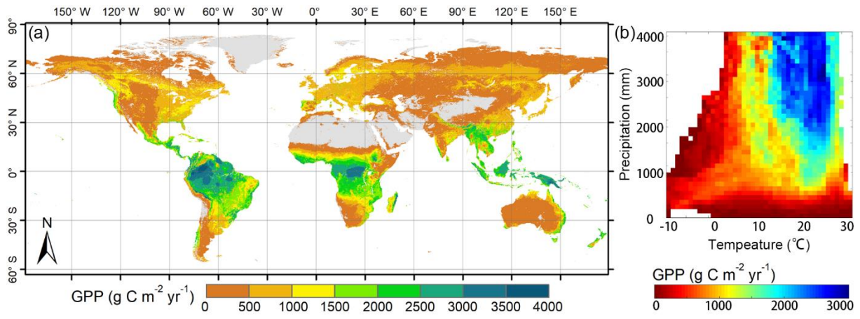
810 Figure 5: Spatial pattern of global GPP simulated by the revised EC-LUE model during 1982–2017: (a) averaged annual GPP, (b) averaged annual GPP at different temperature and precipitation gradients.
