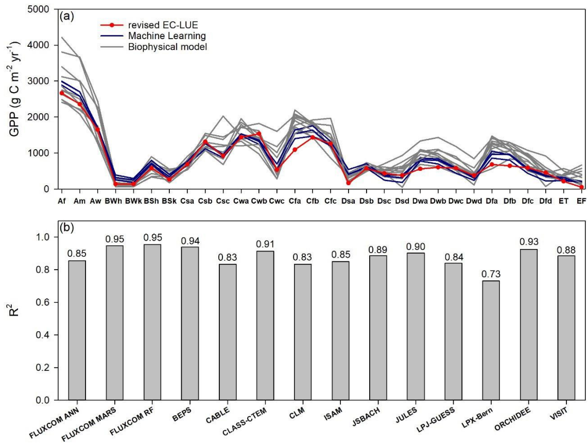
830 Figure 79: Comparisons of long-term (1982 to 2010s) averaged GPP between the revised EC-LUE model and other models across 835 bioclimatic zones in the Köppen-Geiger climate classification map (Beck et al., 2018). (a) the regional averaged value (b) correlation 840 coefficients ( R^2 ) of GPP across all the bioclimatic zones between the revised EC-LUE model and other models. These models including machine learning models (FLUXCOM ANN, FLUXCOM MARS, FLUXCOM RF; Jung et al., 2017), biophysical models BEPS (Ju et al., 2006; Liu et al., 2018), and ten biophysical models in TRENDY (CABLE, CLASS-CTEM, CLM, ISAM, JSBACH, JULES, LPJ-GUESS, LPX-Bern, ORCHIDEE, and VISIT). The abbreviations for the bioclimatic zones are as follows: Af, tropical, rainforest; Am, tropical, monsoon; Aw, tropical, savannah; BWh, arid, desert, hot; BWk, arid, desert, cold; BSh, arid, steppe, hot; BSk, arid, steppe, cold; Csa, temperate, dry summer, hot summer; Csb, temperate, dry summer, warm summer; Csc, temperate, dry summer, cold summer; Cwa, temperate, dry winter, hot summer; Cwb, temperate, dry winter, warm summer; Cwc, temperate, dry winter, cold summer; Cfa, temperate, no dry season, hot summer; Cfb, temperate, no dry season, warm summer; Cfc, temperate, no dry season, cold summer; Dsa, cold, dry summer, hot summer; Dsb, cold, dry summer, warm summer; Dsc, cold, dry summer, cold summer; Dsd, cold, dry summer, very cold winter; Dwa, cold, dry winter, hot summer; Dwb, cold, dry winter, warm summer; Dwc, cold, dry winter, cold summer; Dwd, cold, dry winter, very cold winter; Dfa, cold, no dry season, hot summer; Dfb, cold, no dry season, warm summer; Dfc, cold, no dry season, cold summer; Dfd, cold, no dry season, very cold winter; ET, polar, tundra; EF, polar, frost.
