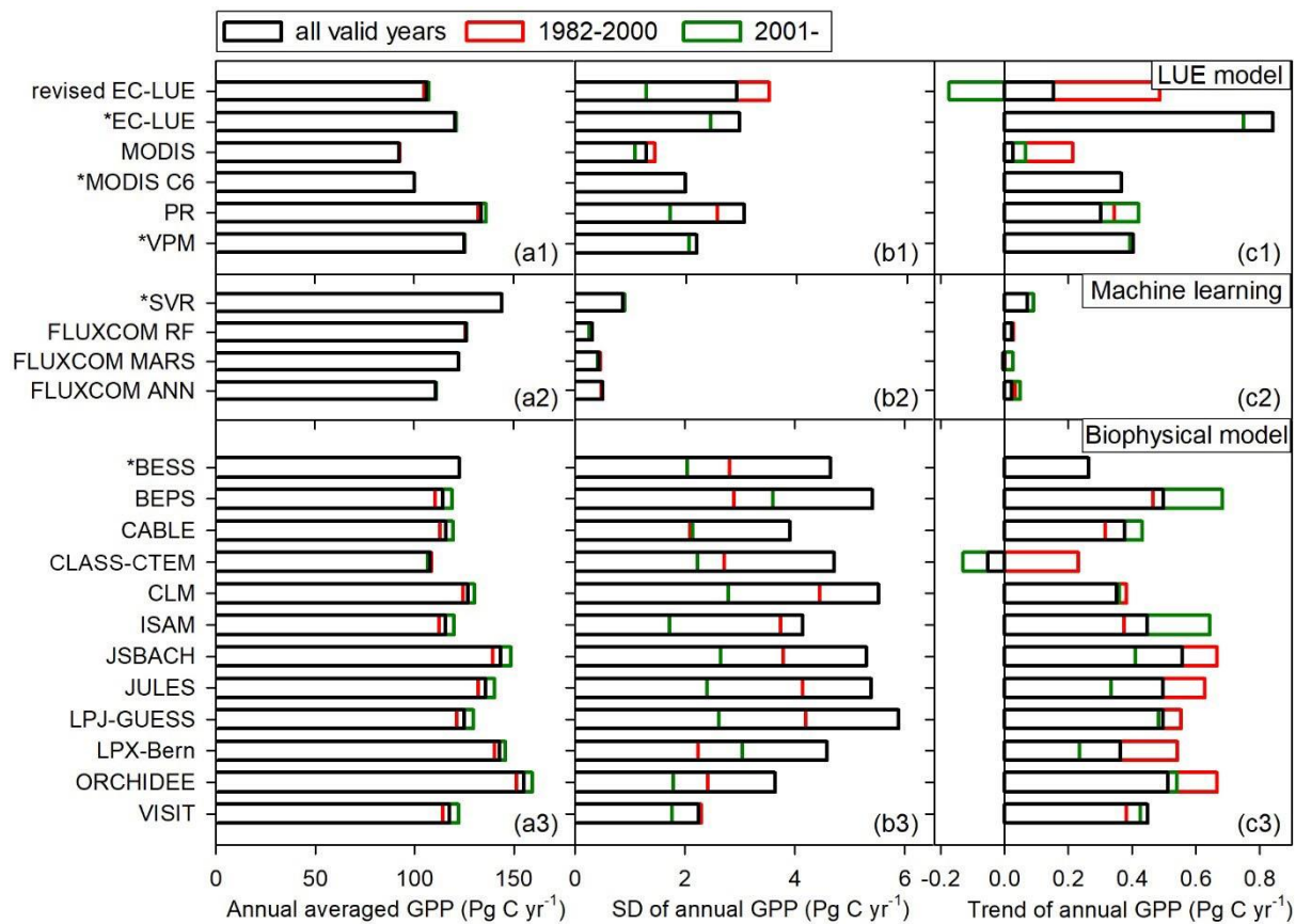
Figure 9.11: Comparison of (a1)–(a3) averaged annual GPP, (b1)–(b3) interannual variability in annual GPP represented by standard deviation (SD), and (c1)–(c3) annual GPP trend among different GPP datasets or models. The references of these models are the same as in Figure 9. * indicates that the valid period of the dataset begins from 2000 or 2001.
