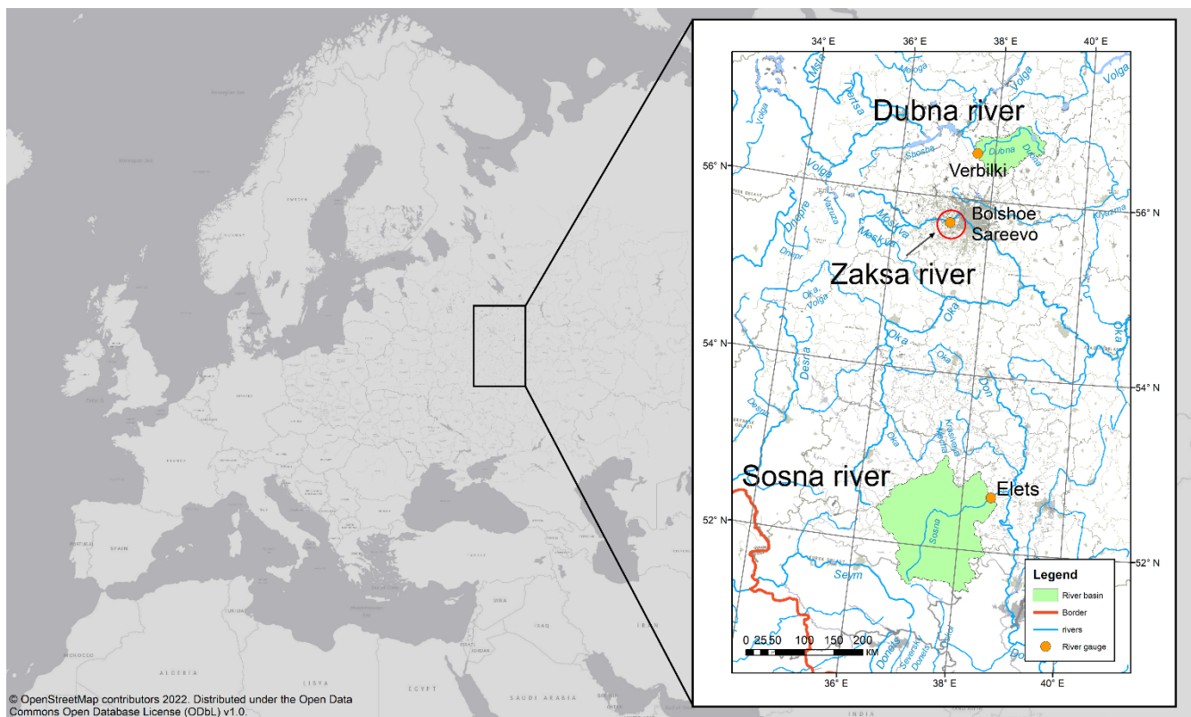
Figure 1: Location of three river basins in the center of the East European Plain.
