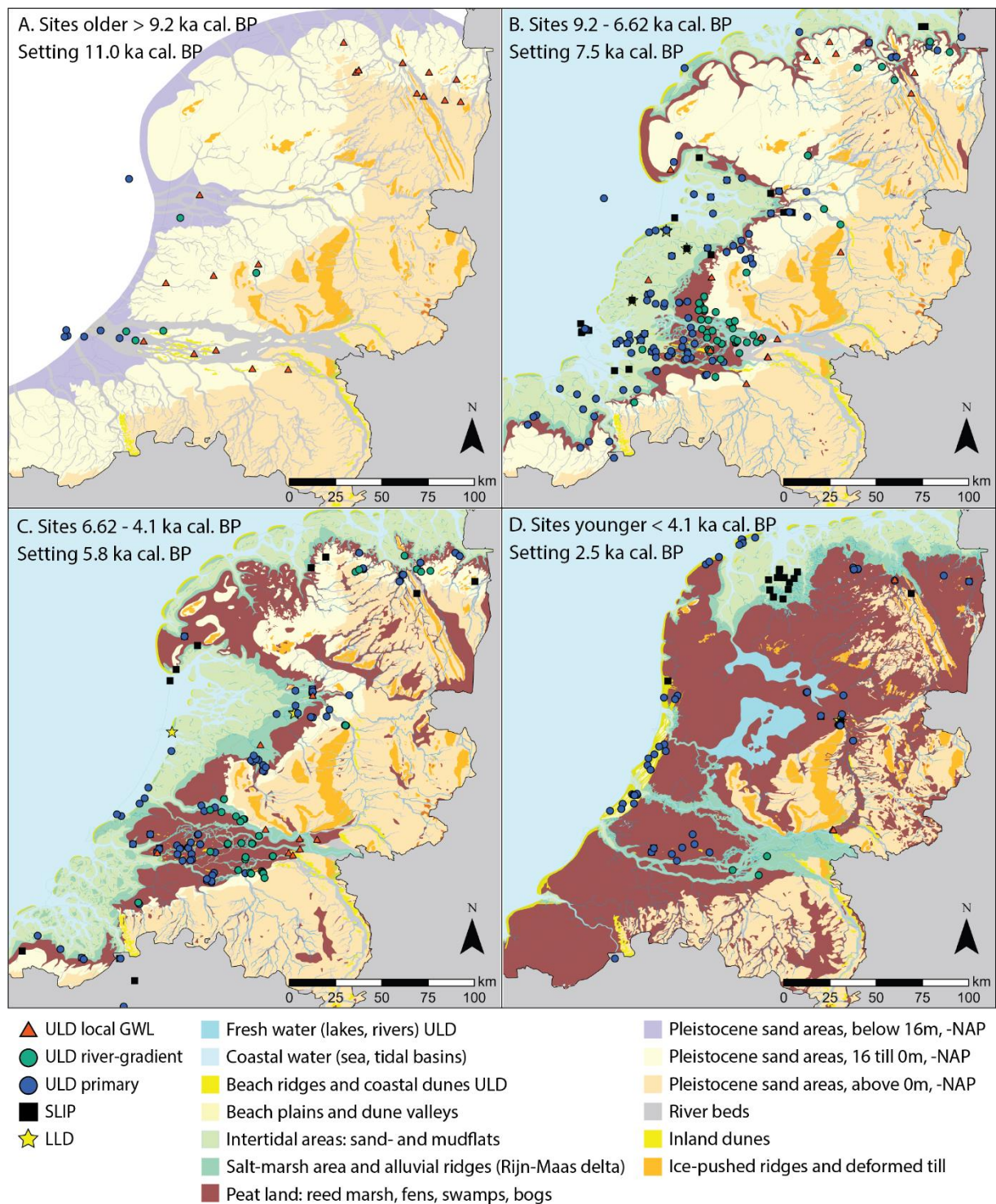
130 Figure 2 Geological water-level indicator site locations (this paper and data set) plotted over a national palaeogeographical map series (Vos et al., 2020), split for four time slices. The indicators shown have an age surrounding the date stamp of each selected map.
