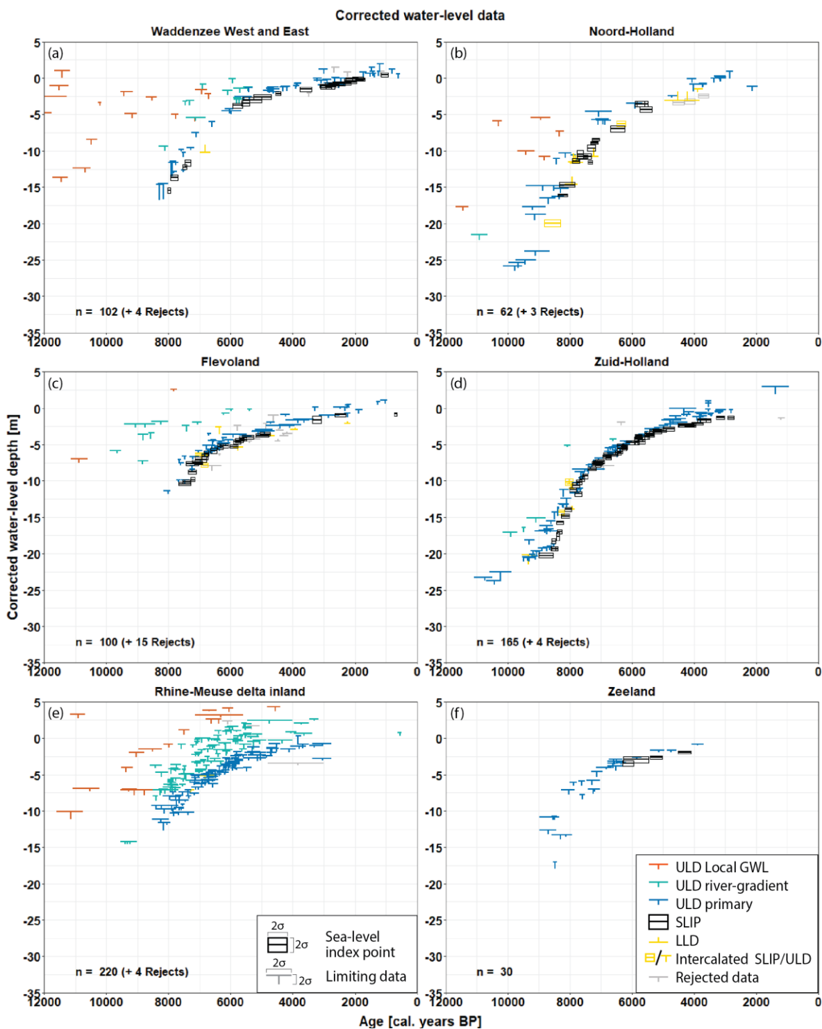
Figure 9 Age-depth plots of the corrected water level elevation for geological indicators per subregion from 12 to 0 ky cal. BP
