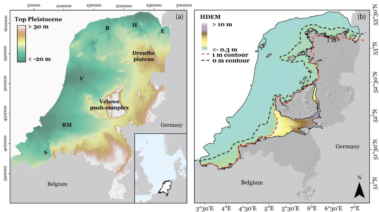
Figure 1 (a) Digital elevation model of the top of Pleistocene deposits, corrected for Holocene erosion (Cohen et al., 2017b, a; Koster et al., 2017). The labels show the location of several palaeo-valleys, B: Boorne, H: Hunze, E: Ems, V: Vecht, RM: Rhine-Meuse, S: Scheldt; (b) High stand digital elevation model (HDEM), regional groundwater table surface reconstructed for 1000 cal. yr. BP (Cohen, 2005; Cohen et al., 2017a, b; locally modified). The 0 m MSL contour (black dashed) and +1 m MSL contour (red dashed) are shown. The study area contour is adopted from Pleistocene landform outlining in national geomorphological and archaeological landscape mapping (as in Cohen et al., 2017a, b) and outside the Rhine-Meuse delta roughly coincides with the +1 m elevation contour line. Projection: RD (EPSG 28992)
