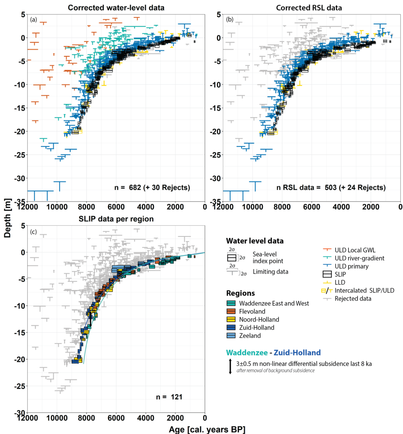
705 Figure 10 Age of indicator data plotted against various sample elevations based on different vertical adjustments applied: (a) Using the indicative water-level, and corrected for decompaction, background basin subsidence and anthropogenic deep subsidence; (b) As A but incorporating a palaeotidal correction for SLIPs and removing secondary ULD and rejected samples (both in grey); (c) Fully processed SLIP data (all vertical corrections considered), coloured by Region, with tentative curves for the Waddenzee (light blue) and Zuid-Holland SLIP data (dark blue) to illustrate deviation back in time.
