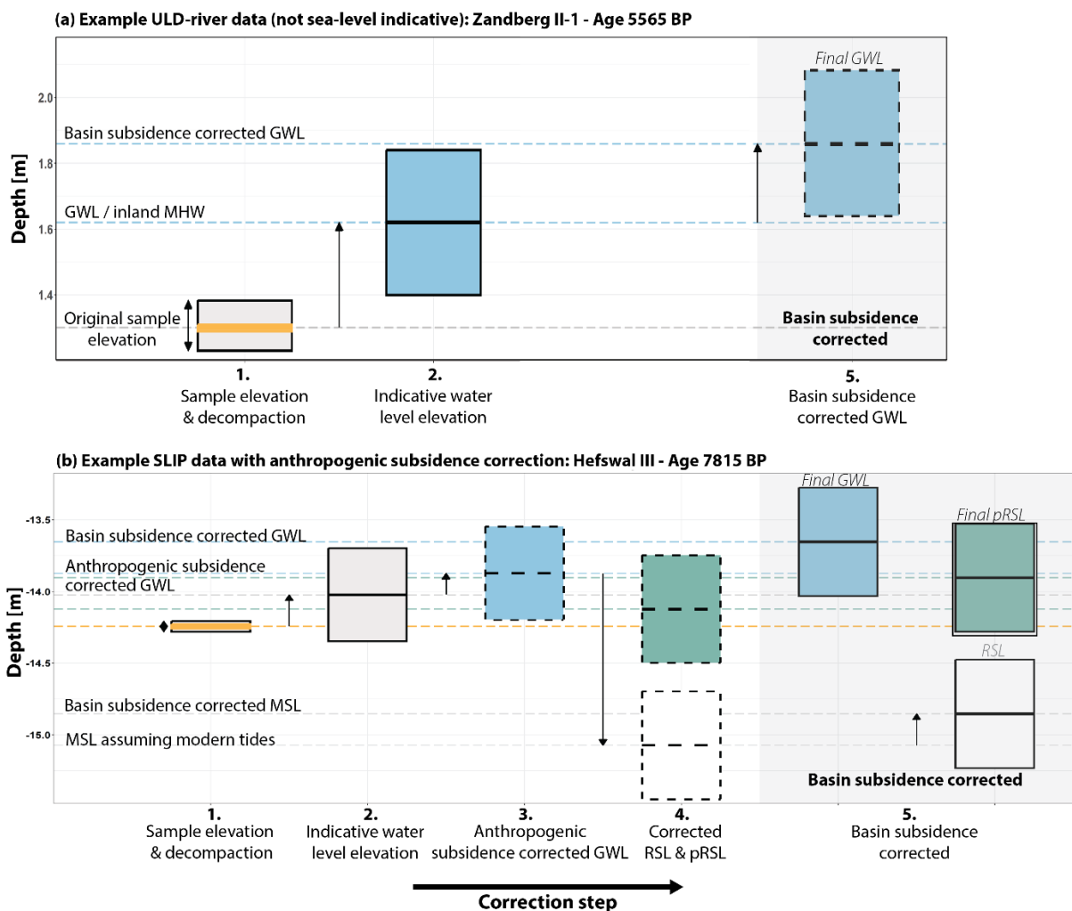
545 Figure 5 Dashboard of sample elevations of two example samples for visual inspection of vertical positioning owing to vertical 550 correction steps. (a) Inland GWL / Upper limiting sample without anthropogenic subsidence, (b) Fen peat SLIP sample from the 555 northeast of the Netherlands, affected by deep anthropogenic subsidence
