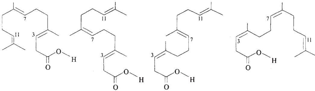
3,7-trans/trans- isomer
