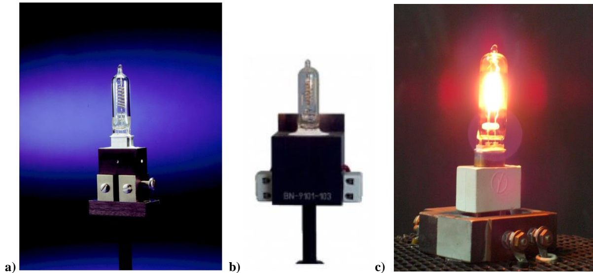
Figure 1. The three main types of FEL tungsten halogen lamps: a) Gooch and Housego OL FEL 1000 W, source Gooch and Housego; b) Gigahertz BN-9101 FEL 1000 W, source Gigahertz-Optik; c) Gamma Scientific Model 5000 FEL 1000 W, source Gamma Scientific.
