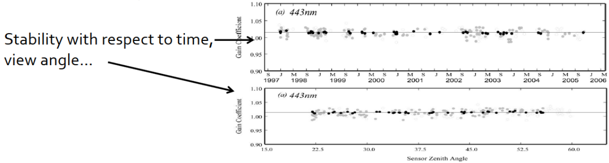
Figure 6: SeaWiFS gains derived from BOUSSOLE (from Franz et al., 2007).
