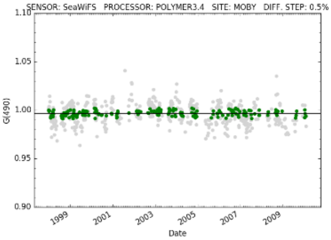
Figure 47: POLYMER gain time series at 490 computed on MOBY.
