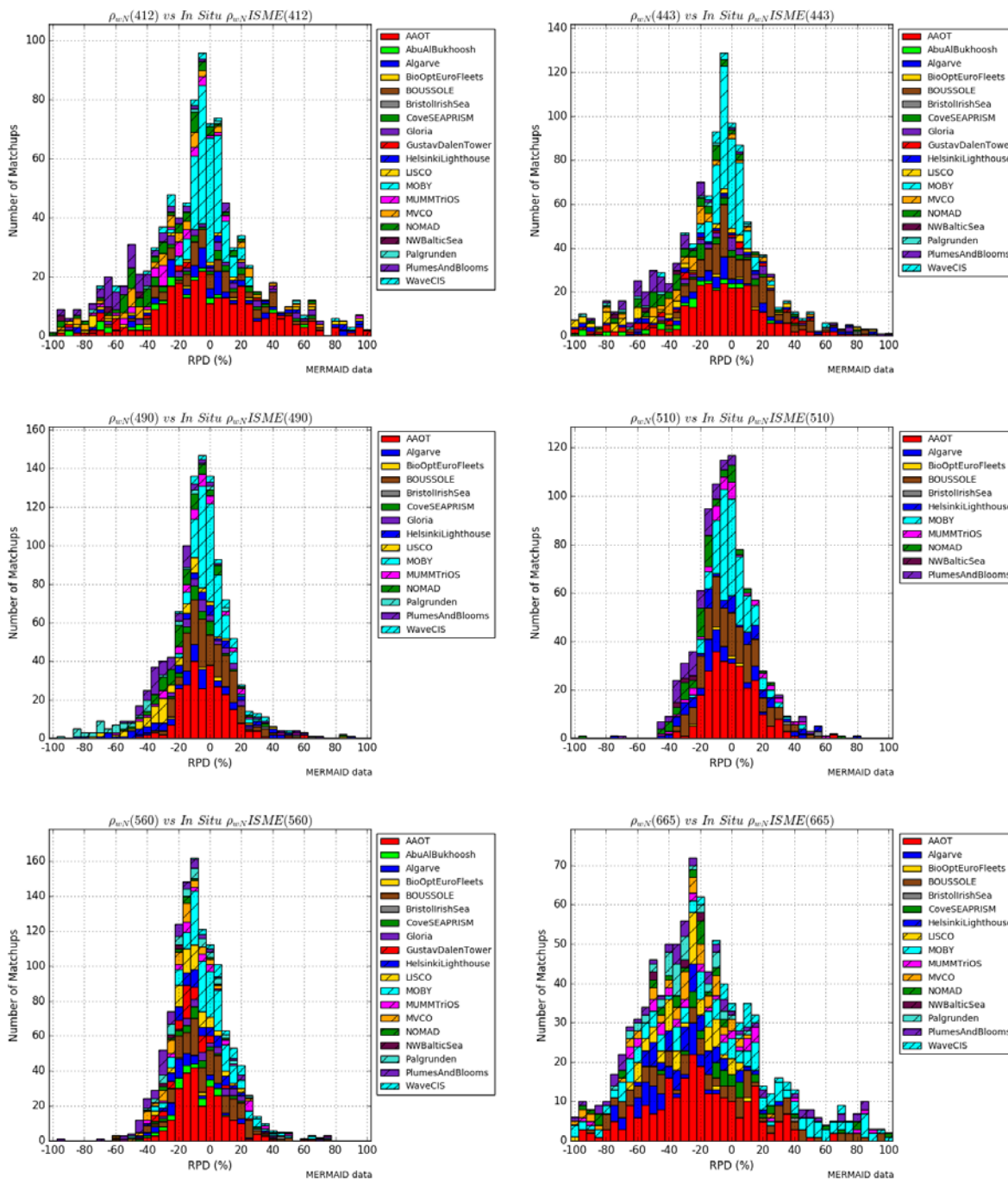
Figure 46: Relative percent differences of water-leaving reflectance between MERIS 4th reprocessing data and in situ data between 412 nm and 665 nm.
