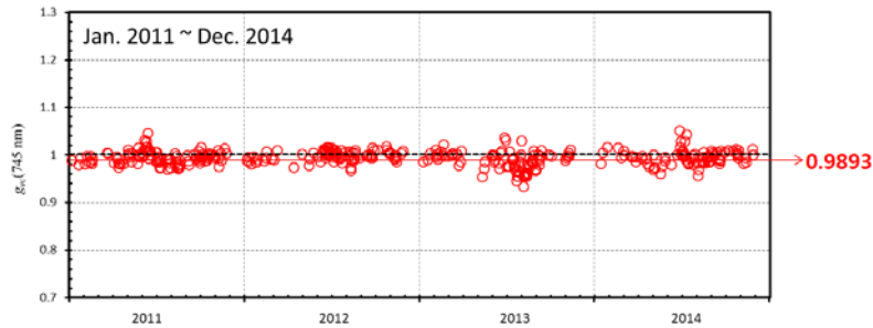
Figure 52: GOCI NIR gain time series at 745nm.
