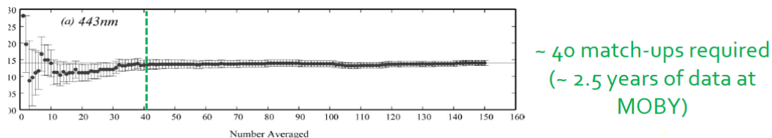
Figure 7: Number of matchups required to derived stable gains (from Franz et al., 2007).
