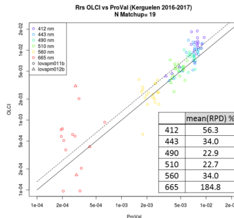
Figure 43: The 19 OLCI matchups with two ProVal obtained in six months in the Kerguelen area. The mean relative percentage deviation for each band is displayed too.
