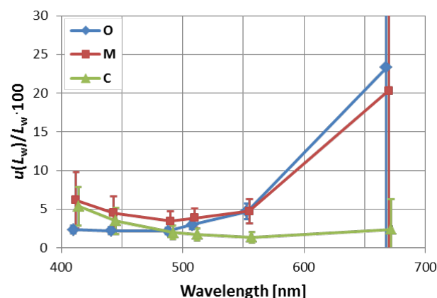
Figure 15: Relative uncertainties u(L_w)/L_w determined assuming a spectrally independent 0.3% uncertainty value for L_T and the mean values of t_a \cdot L_w/L_T for different water types (from Zibordi et al. 2015).
