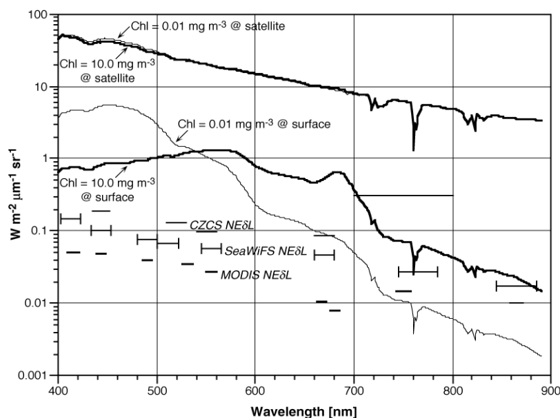
Figure 2 : Space borne sensor sensitivities compared to water-leaving radiance, and radiances measured at the satellite over cloud-free oceans according to model results (from Gordon 1982).
