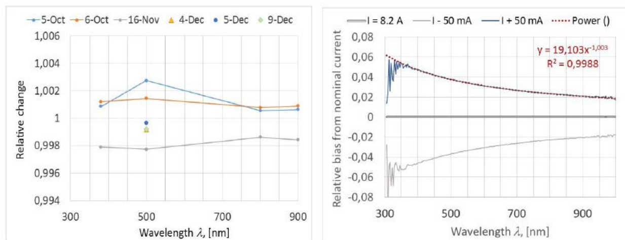
Figure 23: Relative change of the photocurrent of a filter radiometer monitoring the FEL left; effect of lamp current offset right.
