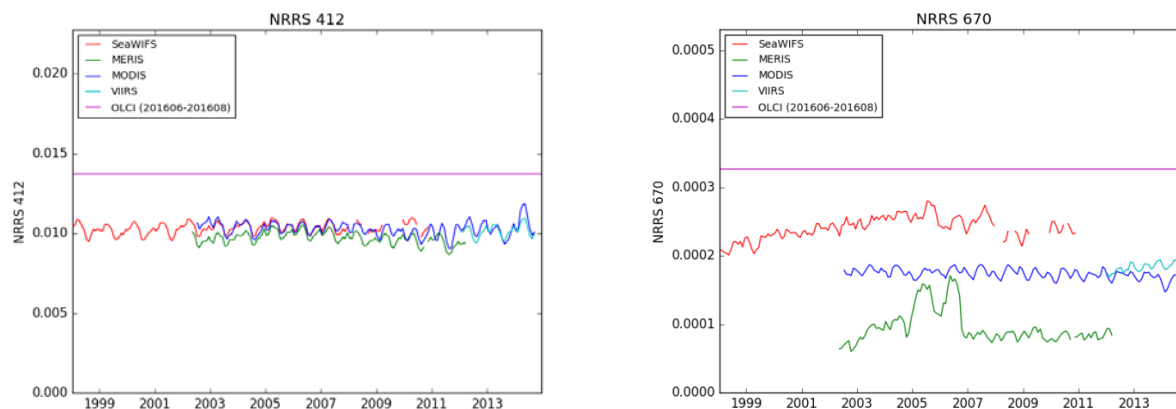
Figure 11: Time-series of (left) NRRS412 and (right) NRRS670 from SeaWiFS, MERIS, MODIS, VIIRS and OLCI.
