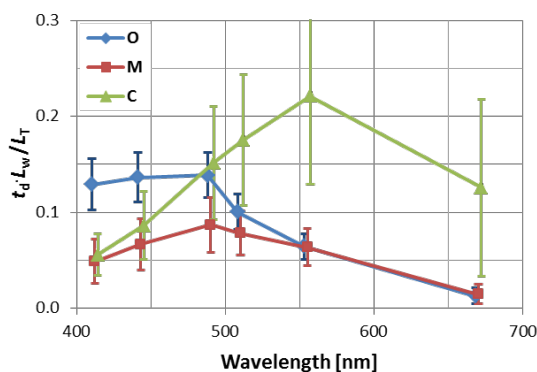
Figure 14: Spectral values of t_d L_w/L_T for oligotrophic (O), mesotrophic (M) and coastal (C) waters. Mean values and standard deviations \sigma (indicated by the vertical error bars), result from the analysis of 814, 1487 and 1045 SeaWiFS data extractions, respectively (from Zibordi et al. 2015).
