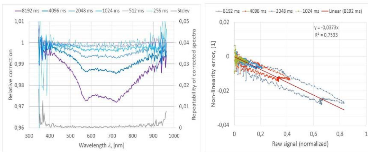
Figure 24: Non-linearity effect as a function of integration time; size of effect and effectiveness of correction left, dependence on the recorded signal amplitude right.
