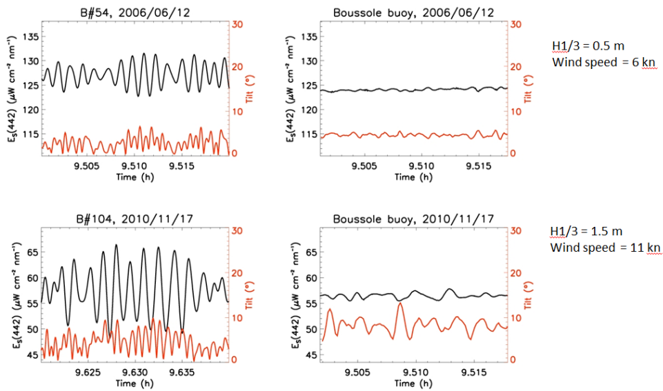
Figure 22: Examples of short (order of minute) contemporary records from ship (left) and buoy (right) surface irradiance at 0.5 m (top) and 1.5 m (bottom) significant wave height (H1/3).
