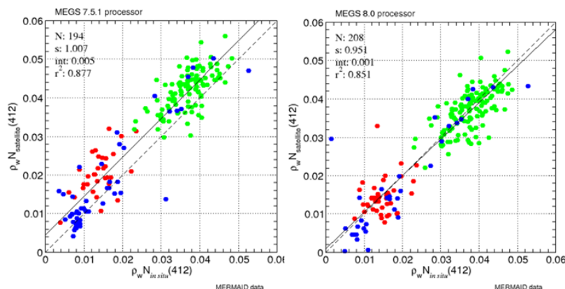
Figure 4: left, MERIS 2nd reprocessing (no SVC); right, MERIS 3rd reprocessing (with SVC). Validation at 412 nm (excluding SVC match-ups); (from Lerebourg et al. 2011, MERIS ATBD).
