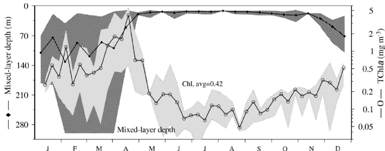
Figure 21: BOUSSOLE seasonal cycle.
