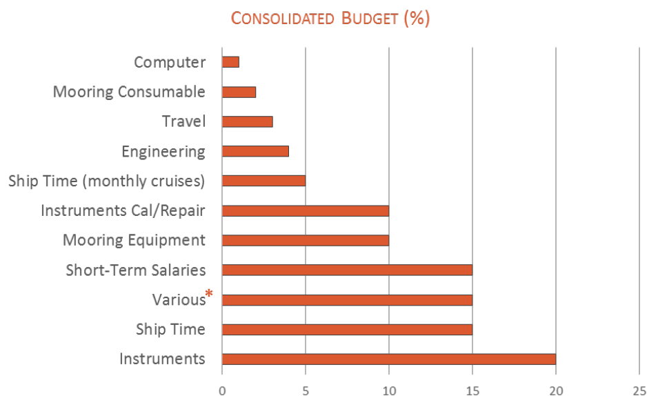
Figure 37: BOUSSOLE consolidated budget (%). Various include: lab levy, cruise instruments, instrument shipping and custom fees, external divers, buoy paint, publications, lab consumable, insurance...
