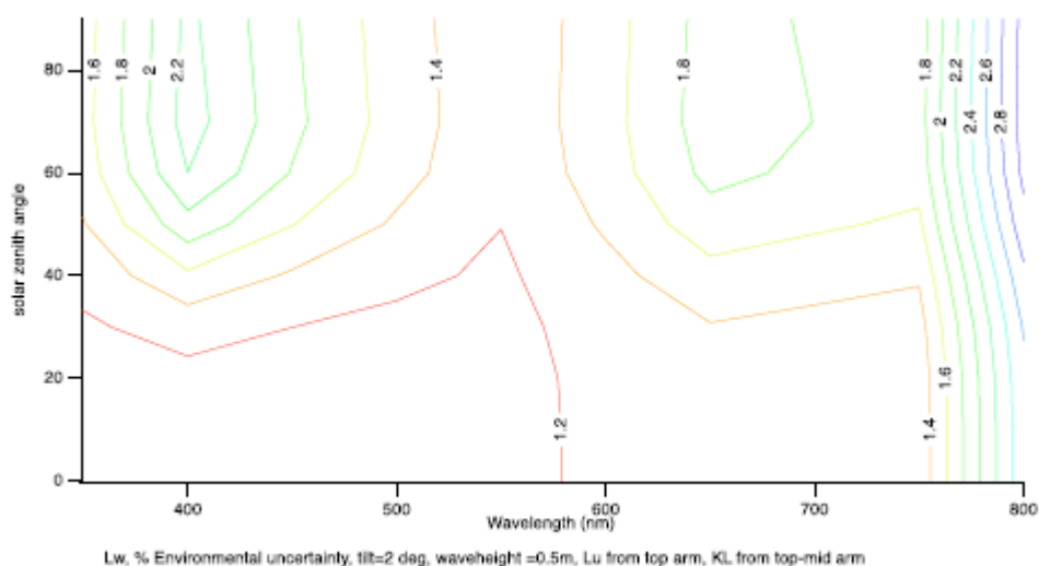
Figure 30: Shows % uncertainty as a function of wavelength and solar zenith angle. Note that the normal reported measurement range for MOBY is currently from 380 nm - 700 nm, and solar zenith angles at the measurement time rarely exceed 55 degrees.
