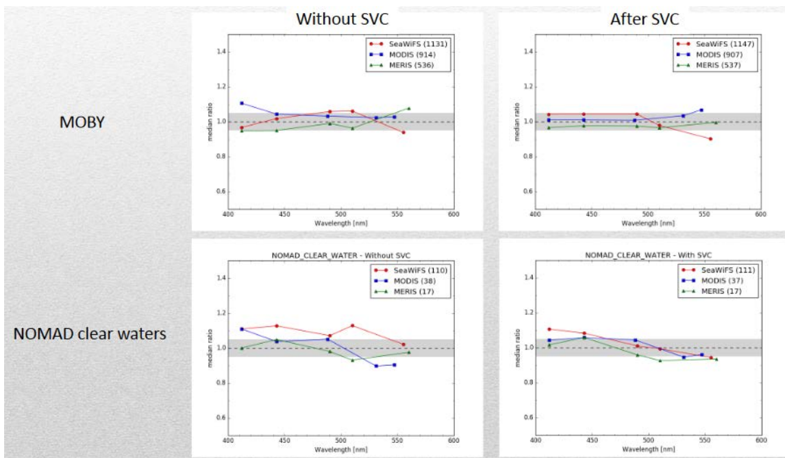
Figure 48: Impact of SVC on sensor harmonisation on clear waters.
