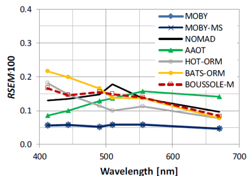
Figure 17: Plot of the standard percent error of the mean (RSEM) for the SeaWiFS g-factors and additionally for MERIS g-factors determined with BOUSSOLE data (i.e., BOUSSOLE-M). (From Zibordi et al. 2015.)
