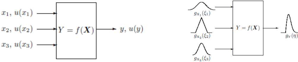
Figure 34: principle of GUM (left) and MCM (right).
