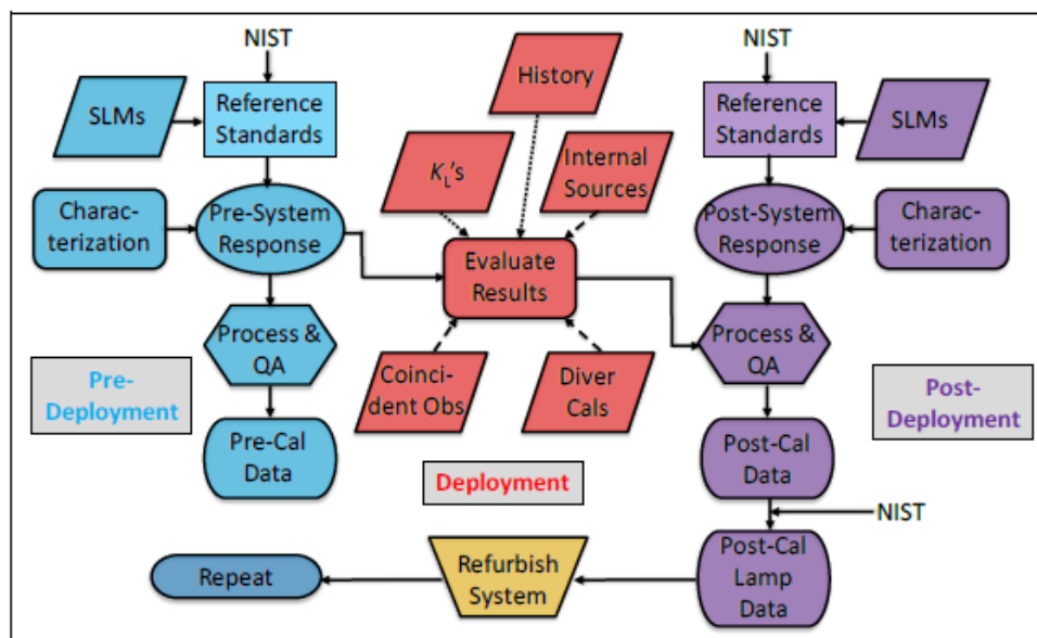
Figure 28: MOBY Radiometric procedures produce values traceable to NIST and generate levels of redundancy as part of the quality assurance program.
