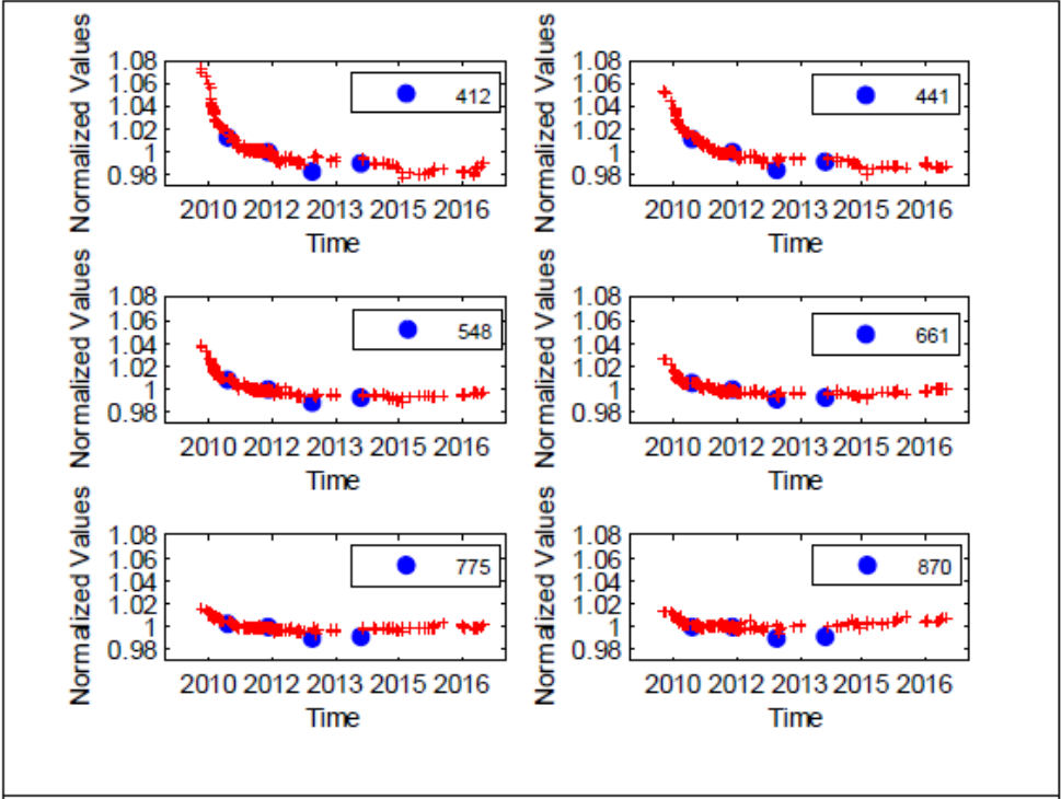
Figure 29: Time series of normalized VXR and FASCAL measurements of the NPR sphere at the VXR spectral bands.
