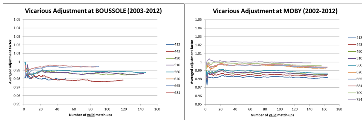
Figure 12: Average MERIS vicarious gain as a function of matchup number. Left: BOUSSOLE (2003-2012), right: MOBY (2002-2012).
