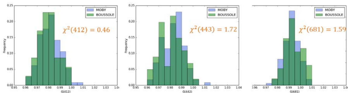
Figure 8: gain distribution derived from BOUSSOLE and MOBY for MERIS 4th reprocessing. (results of C. Mazeran (Solvo) from ESA/IDEAS, N. Lamquin (ACRI-ST) MERIS 4th reprocessing. MERIS data processed with ODESA (ESA/ACRI). MOBY data from Ken Voss (University of Miami) and BOUSSOLE data from David Antoine (CNRS-LOV).
