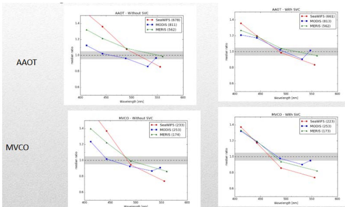
Figure 49: Impact of SVC on sensor harmonisation on AERONET-OC AAOT and MVCO station.
