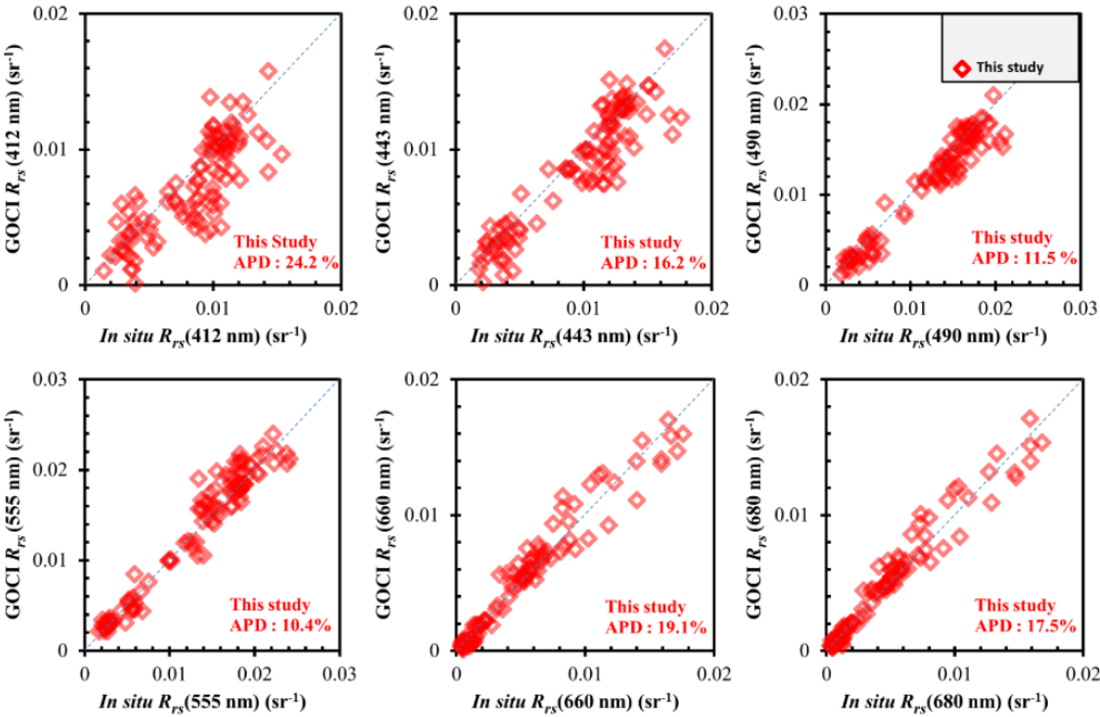
Figure 56: GOCI versus in situ data validation computed AC version 1.5: SRAMS scheme with extended number of aerosol models (Ahn et al., 2016) and water vapour absorption correction at 660, 745, 865nm.
