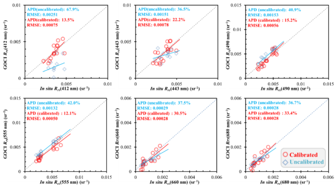
Figure 53: Verification of the vicarious calibration gain factors. Red circles and blue squares represent the GOCI and in situ R_{rs} match – up pairs derived with – and without vicarious calibration, respectively.
