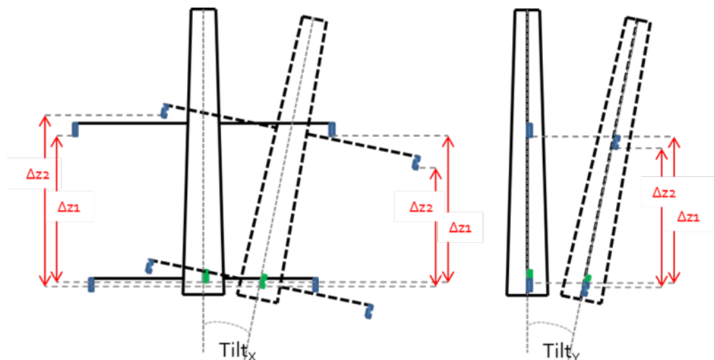
Figure 32: BOUSSOLE tilt correction.
