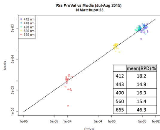
Figure 42: The 23 MODIS matchups with the ProVal obtained in two months at the BOUSSOLE site. The mean relative percentage deviation for each band is displayed too.
