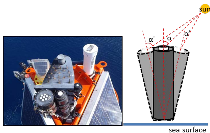
Figure 33: cosine correction of surface irradiance.
