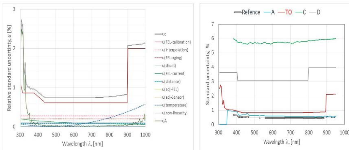
Figure 26: Relative standard uncertainty for calibration of radiance sensors; with uncertainty components evaluated at TO left, uncertainties stated by participants during inter-comparison of radiometers right.
