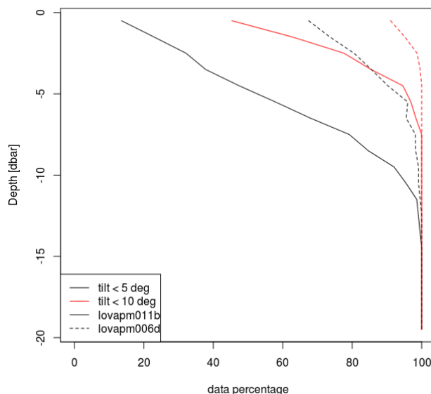
Figure 41: Percentage of data with a tilt below 5° (black line) and 10° (red line) as a function of depth for two floats deployed in the Mediterranean Seas (dotted line) and in the Kerguelen area (solid line).
