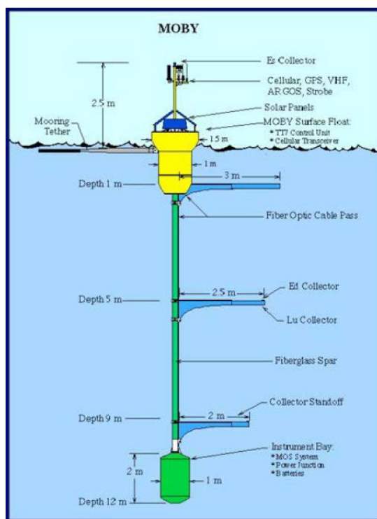
Figure 19: Cartoon illustration of the MOBY buoy.
