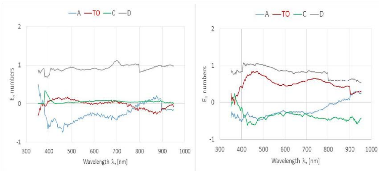
Figure 27: Agreement with the reference value by using E_n numbers; radiance sensor left, irradiance sensor right.
