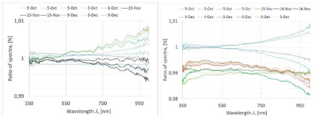
Figure 25: Alignment, non-stability and temperature effects from repeated measurements; radiance sensor left, irradiance sensor right.
