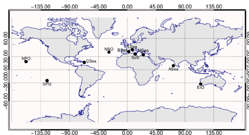
Figure 18: Maritime regions of interest (from Zibordi and Melin, 2017).
