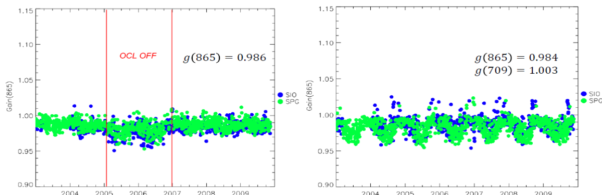
Figure 3: MERIS NIR gain time series over SIO and SPG. Left: methodology developed and implemented for the 3 rd data reprocessing. Two bands used as reference other bands calibrated using a spectral slope model. Right: SeaWiFS like methodology using one NIR band as reference and fixing an aerosol model (MAR90) to calibrate the others. (From Lerebourg et al. 2011, MERIS ATBD).
