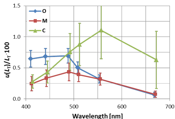
Figure 16: Relative uncertainties u(L_T)/L_T determined assuming a spectrally independent 5% uncertainty value for L_w and the mean values of t_a \cdot L_w/L_T for different water types: oligotrophic (O), mesotrophic (M) and coastal (C). The vertical bars refer to values determined with t_a \cdot L_w/L_T \pm \sigma (from Zibordi et al. 2015).
