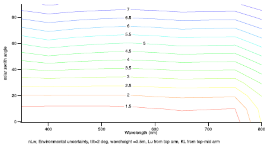
Figure 31: Shows % uncertainty as a function of wavelength and solar zenith angle. Note that the normal reported measurement range for MOBY is currently from 380 nm -700 nm, and solar zenith angles at the measurement time rarely exceed 55 degrees. Still because L_{wn} includes E_s , L_{wn} has increased uncertainty relative to L_w .
