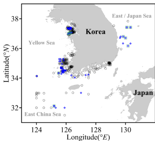
Figure 54: 65 sets of in situ R_{rs} collected from the Korea Ocean Satellite Center (KOSC) cruise campaigns since 2010.
