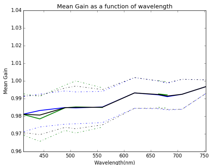
Figure 45: MERIS 4th reprocessing vicarious gains: BOUSSOLE (green), MOBY (blue), and final interpolated gains (black).
