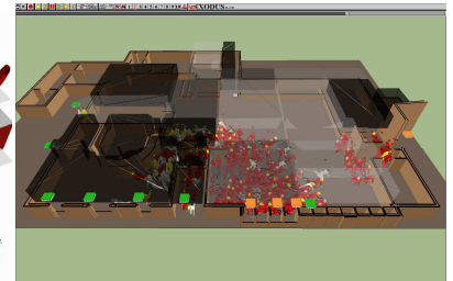
Linked SMARTFIRE and buildingEXODUS simulation of Rhode Island disco fire incorporating smoke, heat, toxic and irritant gases.
