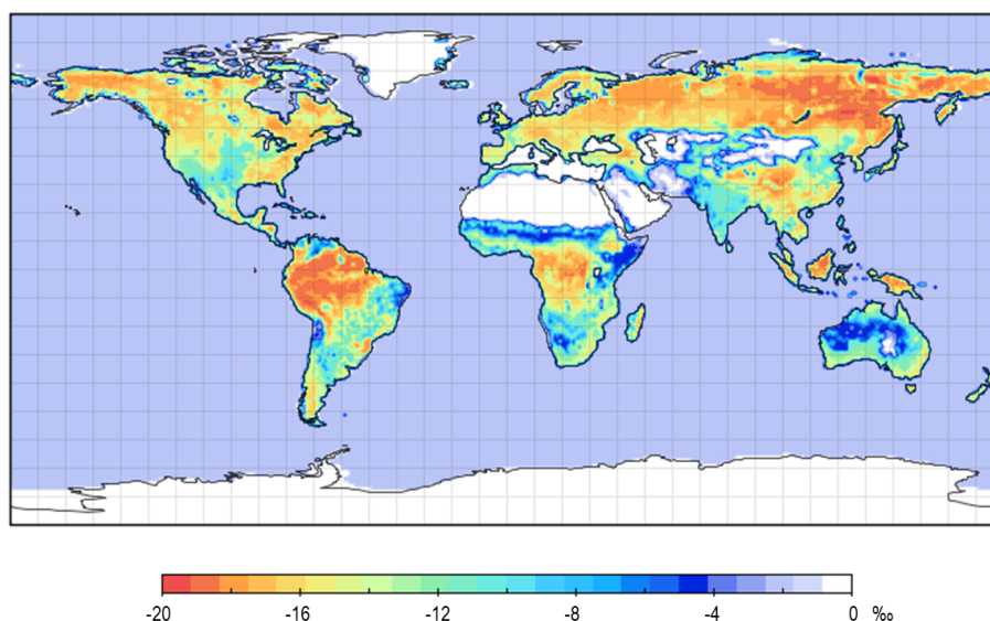
Figure 3. The annual mean of the total photosynthetic {}^{13}\text{C} discrimination ( \Delta in Eq. 7) in 2003.
