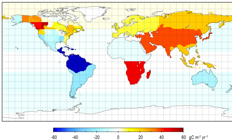
Figure 9. Difference of the inverted \text{CO}_2 flux between using \text{CO}_2 + ^{13}\text{CO}_2 data and using \text{CO}_2 data only (2002–2004 average).
