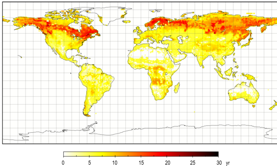
Figure 4. Global distribution of the flux-weighted mean age of soil carbon pools (Eq. 8).
