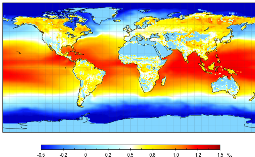
Figure 6. Disequilibria between ^{13}\text{C} fluxes to and from the land or ocean surface in 2000. At the land surface, the disequilibrium is the difference between photosynthetic and respiratory discriminations against ^{13}\text{C} , and at the ocean surface it is the difference in ^{13}\text{C} discrimination between the one-way diffusive downward and upward fluxes.
