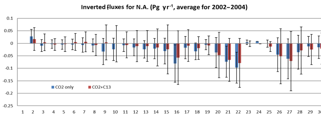
Figure 11. Comparison between inversion results with and without ^{13}\text{CO}_2 constraint for 30 regions in North America.
