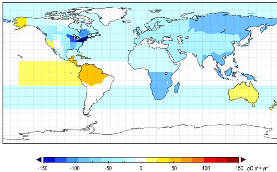
Figure 8. Global distribution of inverted \text{CO}_2 flux using \text{CO}_2 data only (2002–2004 average).
