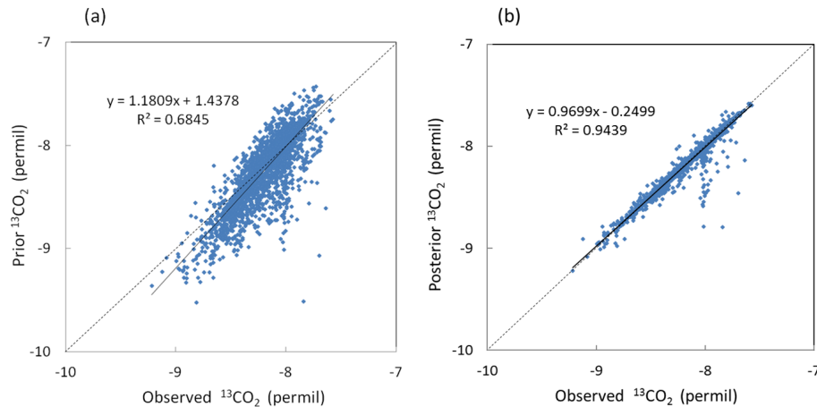
Figure 15. Comparison of prior (a) and posterior (b) ^{13}\text{CO}_2 compositions with observations. The prior composition is obtained through transport modelling with prior ^{13}\text{CO}_2 fluxes from the terrestrial ecosystems, oceans, fossil-fuel emission and biomass burning, and the posterior composition is obtained with the \text{CO}_2 – ^{13}\text{CO}_2 joint inversion (case I).
