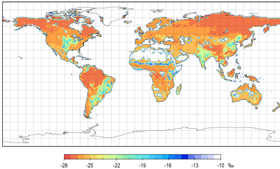
Figure 5. Global \delta^{13}\text{C} distribution over land (annual flux-weighted average in 2003).
