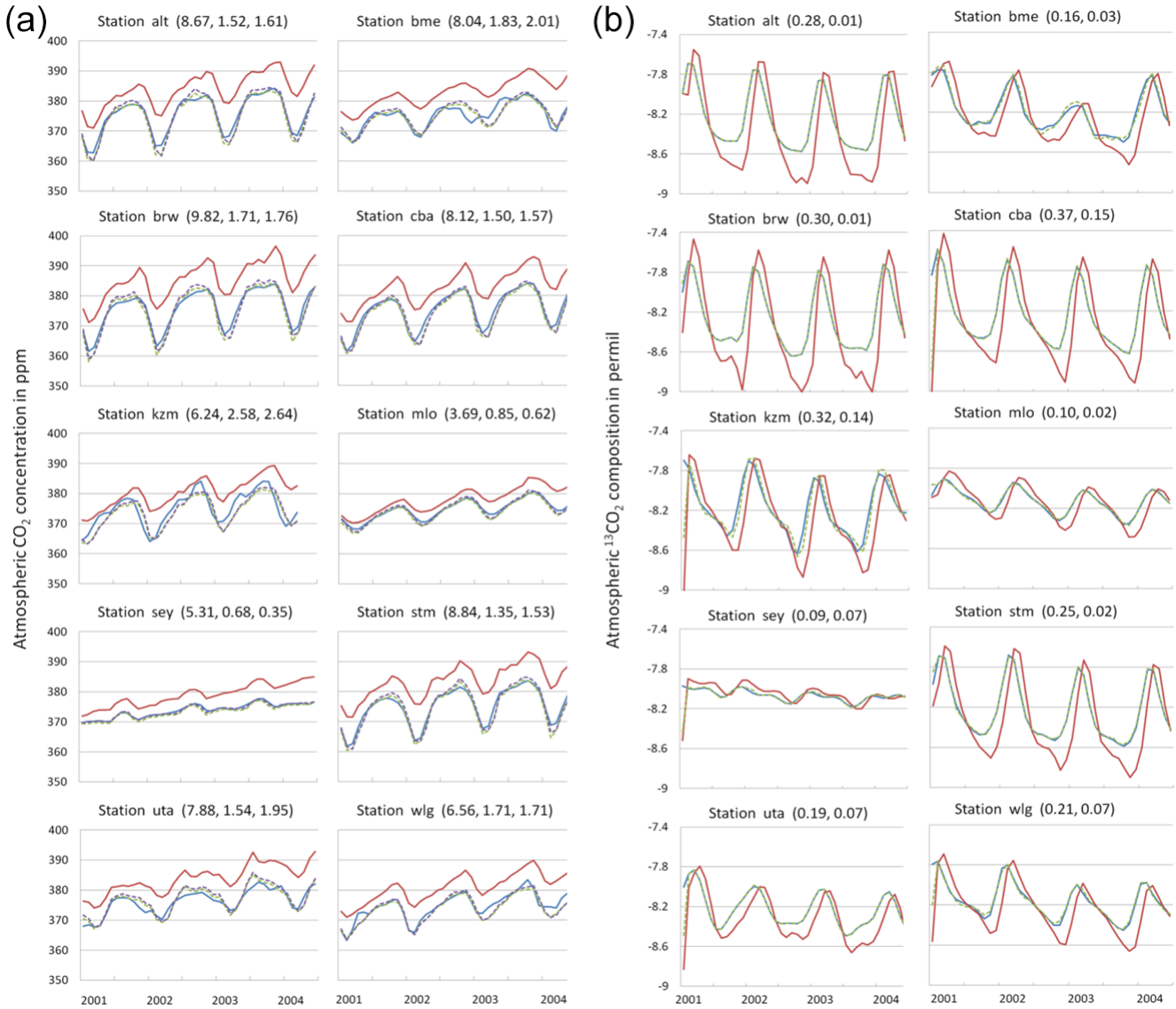
Figure 13. Left panel: comparison of CO 2 concentrations calculated using the prior flux (solid red) and from CO 2 -only inversion (dashed purple) and joint inversion (dashed green) against observations (blue) at 10 randomly selected stations from different regions. The header of each plot indicates the station ID and the root mean square difference (RMSD) for the prior, joint and CO 2 -only inversions against observations. Right panel: comparison of 13 CO 2 composition from the prior (solid red) and joint inversion (dashed green) against observations (blue). The header of each plot indicates the station ID and RMSD of the prior and the joint inversion against observations.
