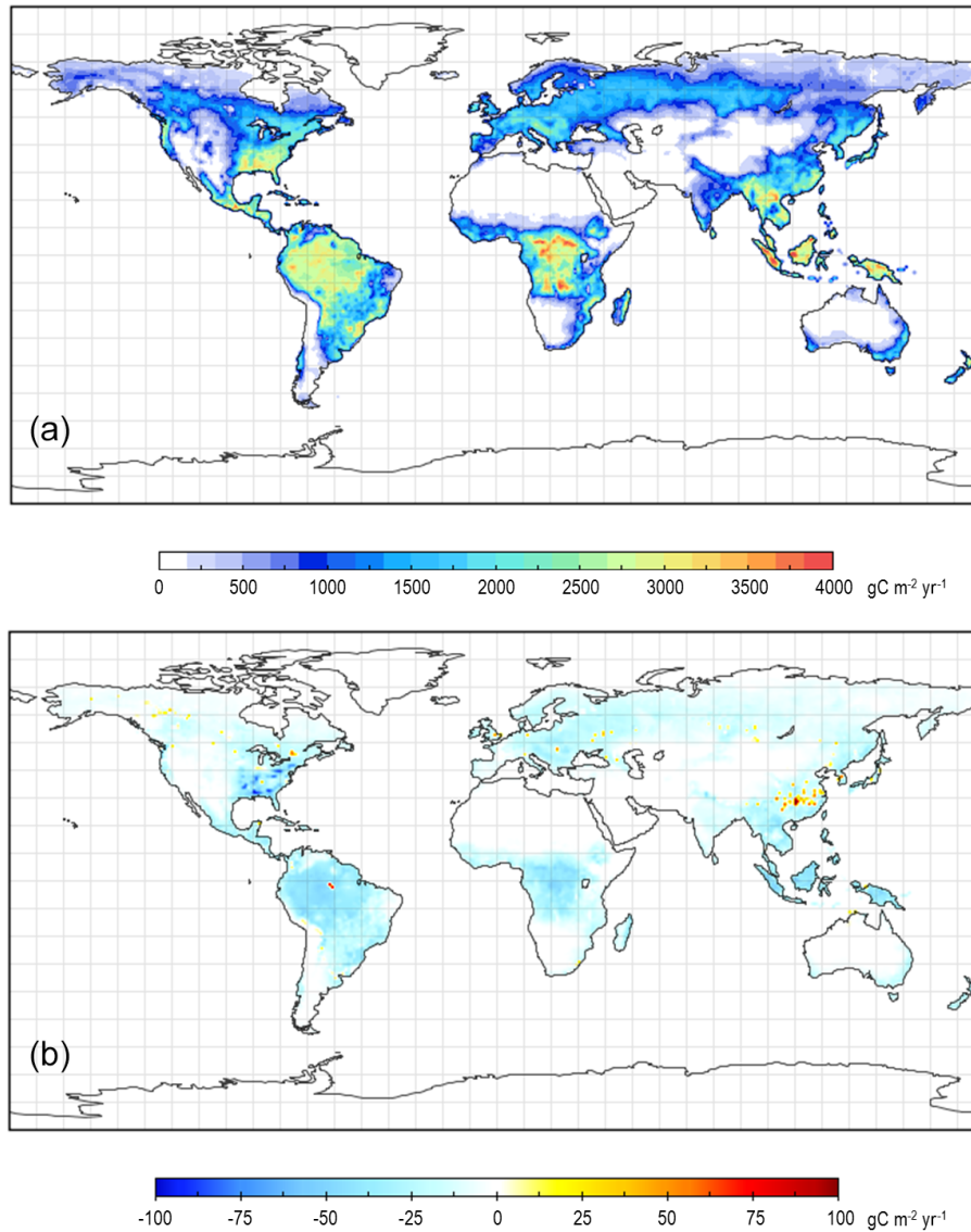
Figure 2. (a) Gross primary productivity (GPP) distribution in 2003 computed using remote sensing LAI and land cover maps and climate and soil data, and (b) net ecosystem productivity (NEP) distribution in 2003. Both are calculated using the BEPS model. Annual NEP maps from 2000 to 2004 are used to as the prior flux in the inversions. This GPP map is used to distribute the flux uncertainty among the 39 land regions.
