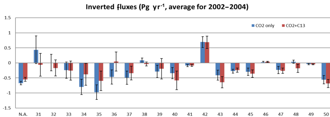
Figure 10. Comparison between inversion results with and without ^{13}\text{CO}_2 constraint for 21 regions of the globe for the periods of 2002–2004.
