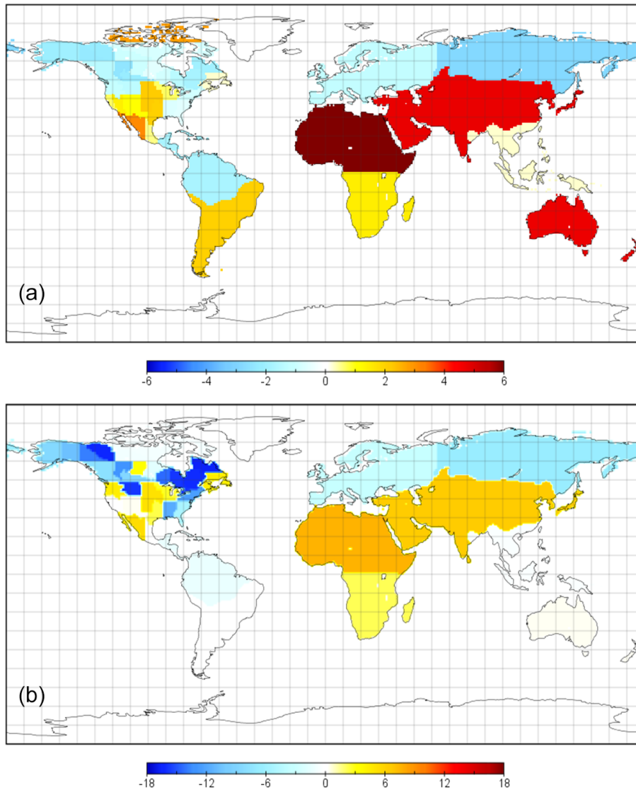
Figure 12. (a) Difference in \varepsilon_{1pH} (‰) and (b) the inverted \text{CO}_2 flux ( \text{g C m}^{-2} \text{ year}^{-1} ) between case I and case II, i.e. Case I minus case II. See Sect. 2.1.3 for the description of these cases.
