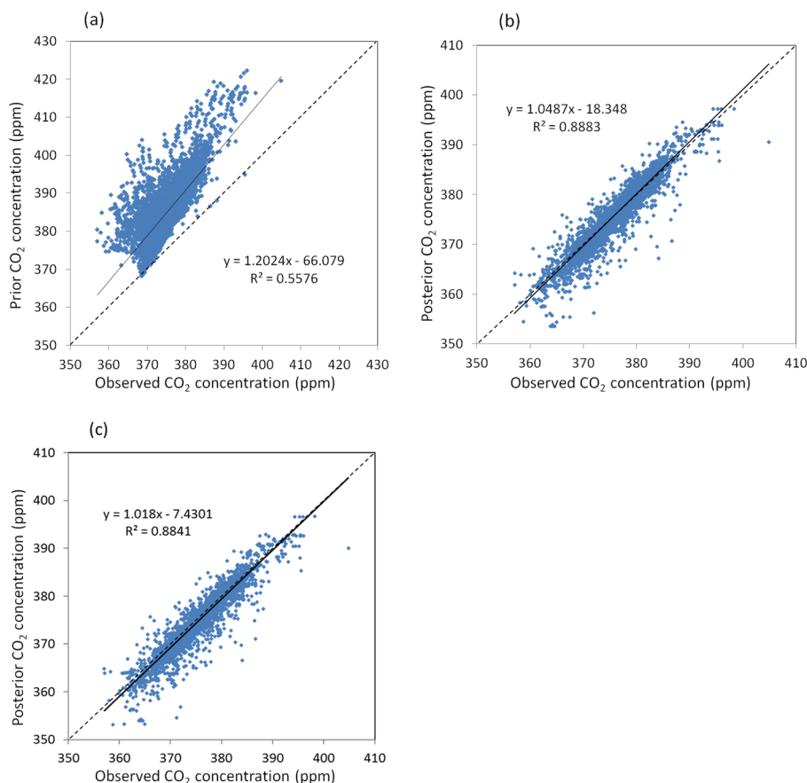
Figure 14. CO 2 concentrations from (a) prior, (b) posterior from the CO 2 -only inversion and (c) posterior from the joint inversion in comparison with observations. The prior concentration is obtained through transport modelling with prior CO 2 fluxes from the terrestrial ecosystems, oceans, fossil-fuel emission and biomass burning.
