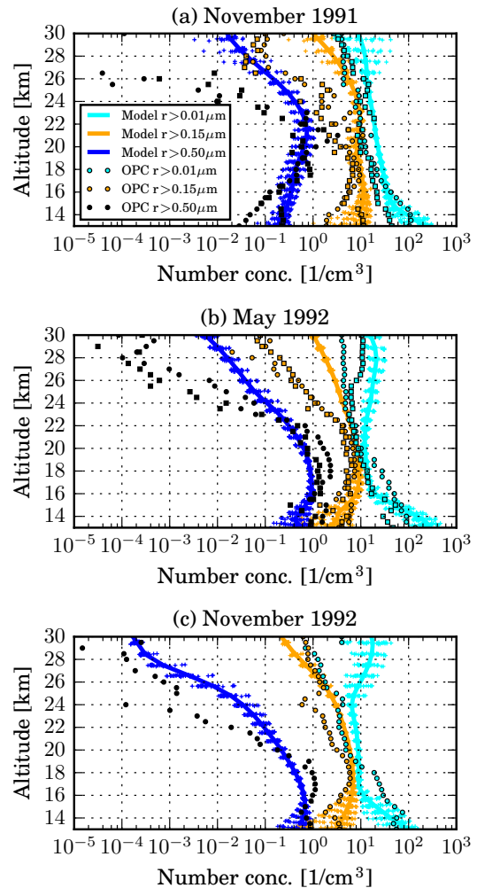
Figure 11. Vertical profile of the cumulative aerosol number concentration ( \text{cm}^{-3} ) for three channels ( r > 0.01\mu\text{m} in light blue, r > 0.15\mu\text{m} in orange, and r > 0.50\mu\text{m} in dark blue) in November 1991, May 1992, and November 1992 at Laramie, Wyoming ( 41^\circ\text{N} , 105^\circ\text{W} ), in the style of Sekiya et al. (2016). Solid lines show the modelled monthly mean, while the crosses indicate the range of daily mean concentrations within that month. Optical particle counter (OPC) measurements from Deshler et al. (2003) are shown as symbols.
