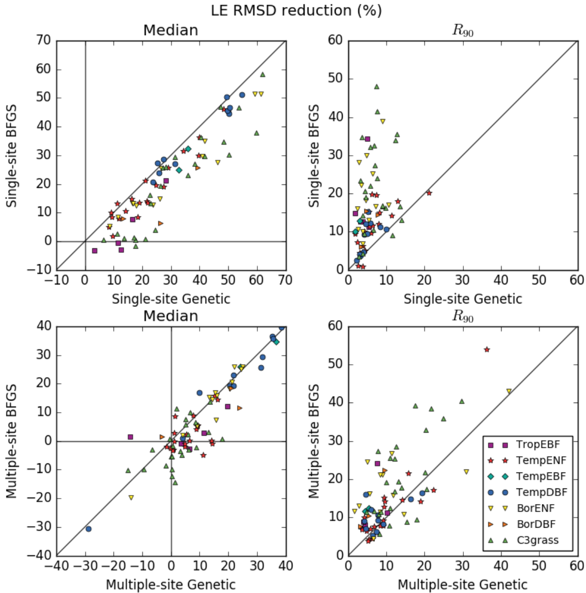
Figure S2: Comparison of the performances between the gradient-based and genetic methods in terms of model–data RMSD reduction (%) obtained for the daily LE fluxes. The left panels show the medians across the results obtained within 16 optimisation tests with random first-guess parameter values for each site; the right panels – the spreads between the 5th and 95th percentiles ( R_{90} ) of the same distributions.
