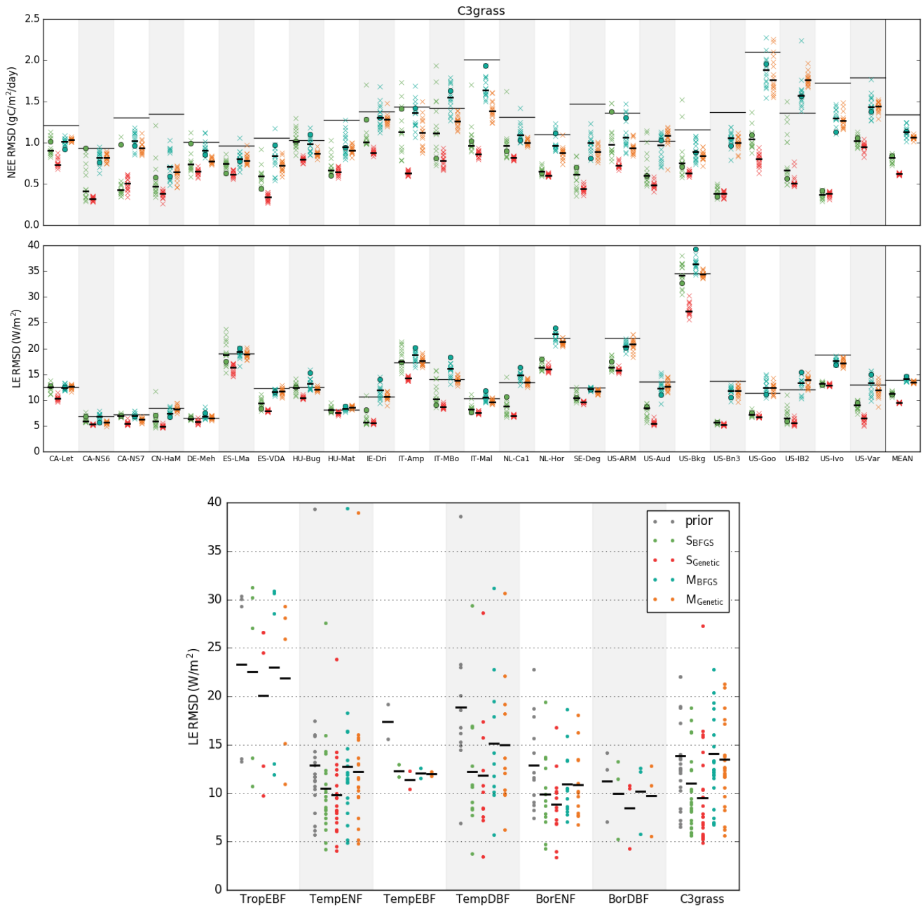
Figure S1: Model–data RMSD for the daily NEE (upper panels) and LE (lower panels) flux time series smoothed with a 15-days moving-average window obtained at different FLUXNET sites with the four optimisation schemes: single-site BFGS (green), single-site genetic (red), multi-site BFGS (blue) and multi-site genetic (orange). Each optimisation is done starting from the 16 different first-guess parameter values (shown by crosses), one of which corresponds to the standard ORCHIDEE values (shown by circles for BFGS). The median values are indicated by the short horizontal bars, the prior model–data RMSD values – by the long horizontal bars. The graphs are grouped by PFTs with the last column showing the mean values for the PFT averaged across the sites for each first-guess parameter set. The graph for TempDBF also shows the influence of data smoothing on the final results. The last panel shows the summary graph for the LE fluxes, similar to the Figure 1 in the main text.
