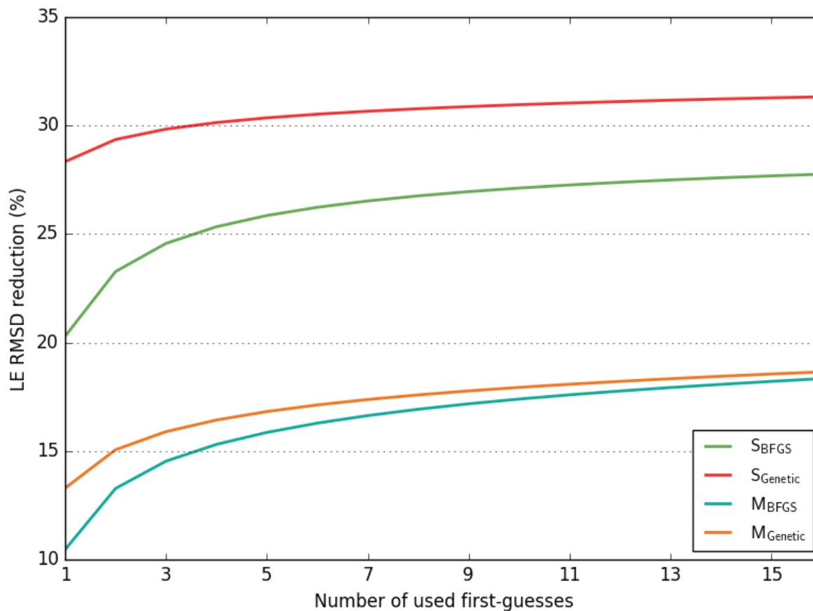
Figure S3: Model–data RMSD reduction (in %) obtained for the LE fluxes as a function of the number of runs performed with random first guess parameter values (for each configuration, S_{BFGS} , S_{Genetic} , M_{BFGS} and M_{Genetic} ). For each number of first guesses (X-axis) all possible combinations across the 16 optimisation tests (i.e. 16 first-guesses) are considered and the maximum RMSD reductions are calculated; the mean of these maximums is reported on the Y-axis. The results are averaged across all sites for each configuration.
