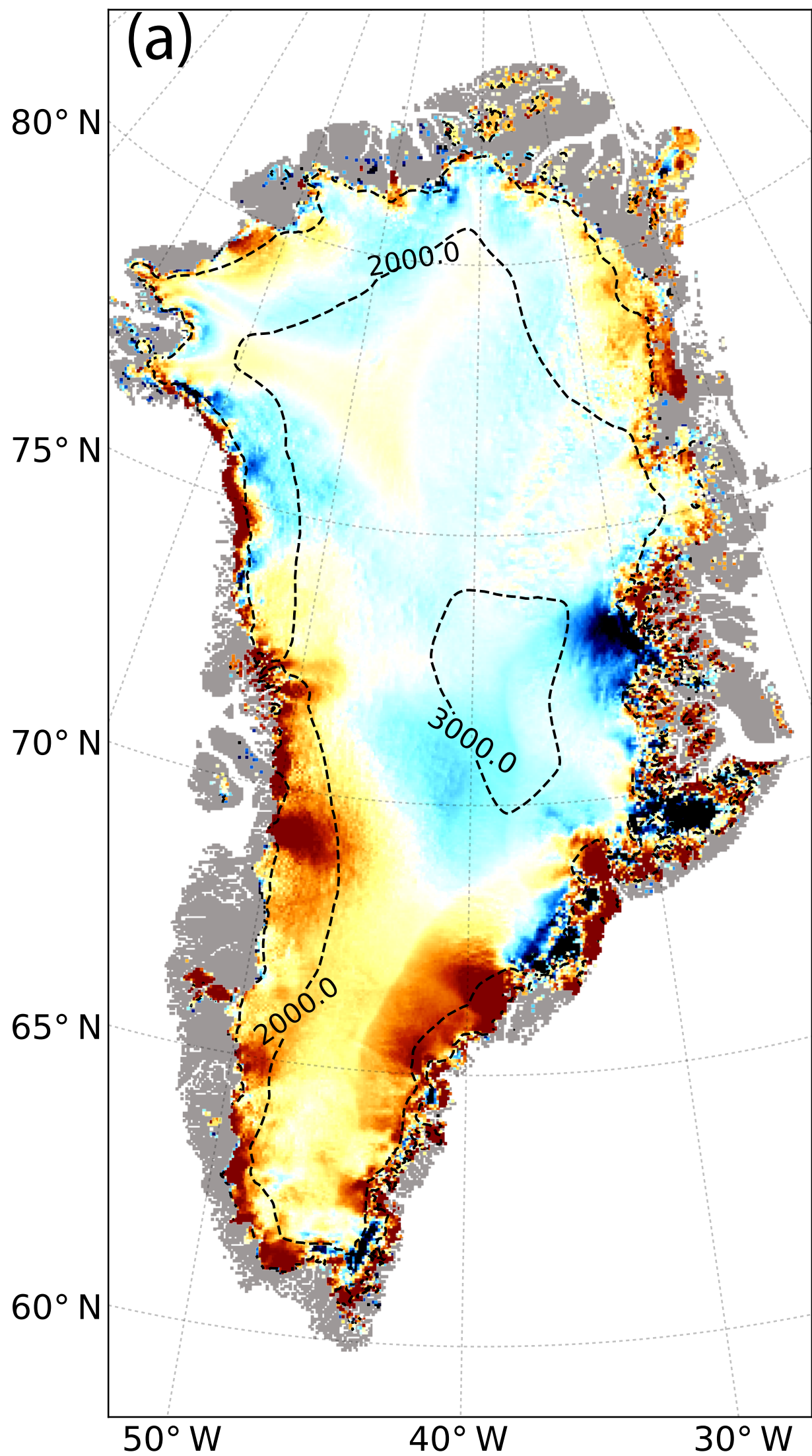
Ice thickness difference (m)
