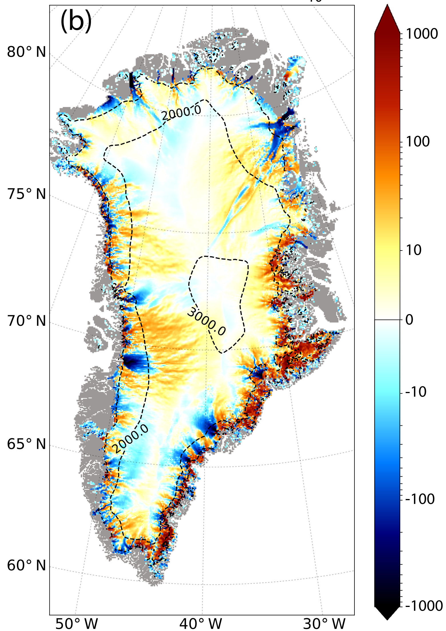
Ice velocity difference ( \text{Log}_{10} m yr -1 )
