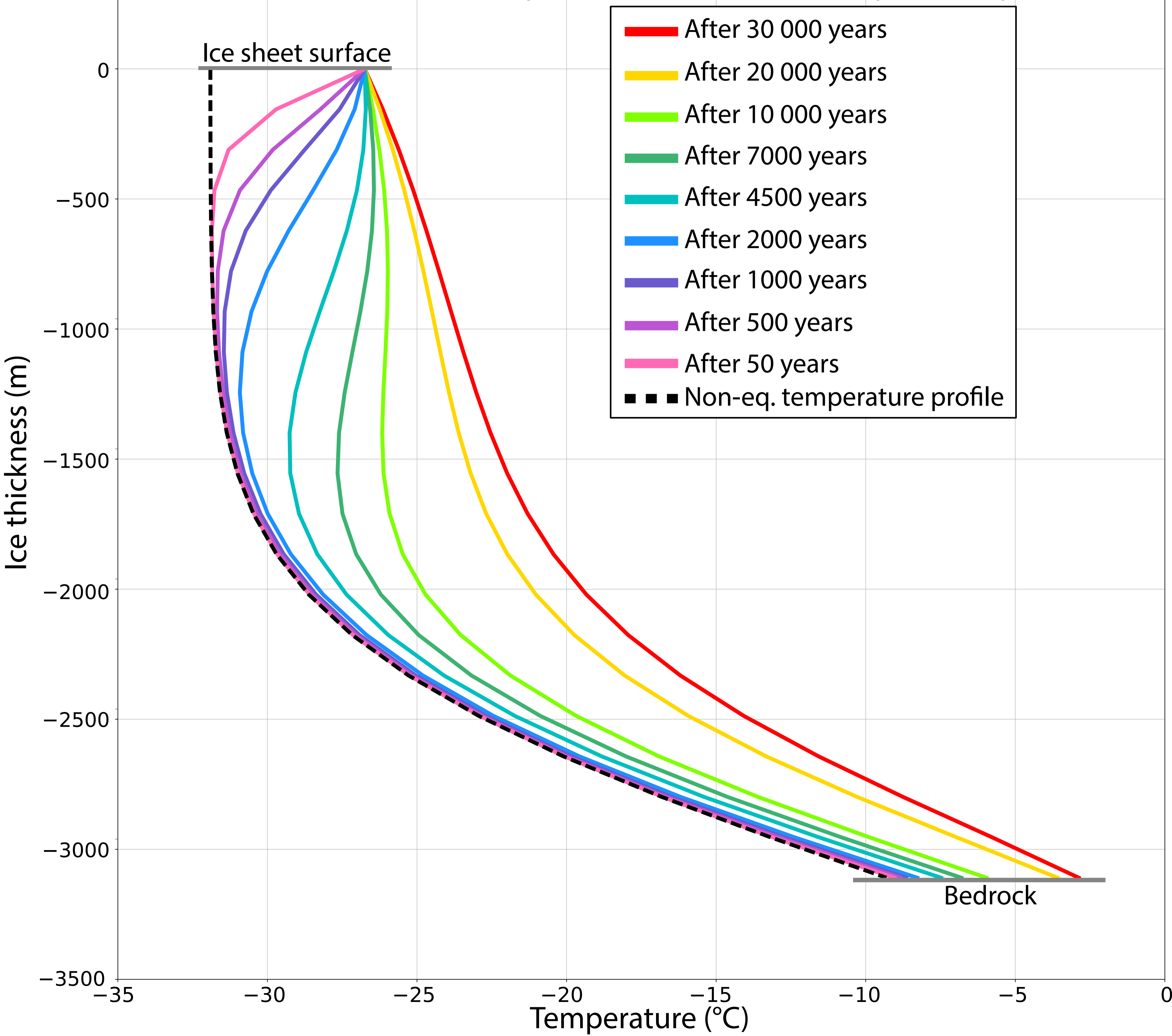
Temporal evolution of verticale ice profile temperature (°C)
