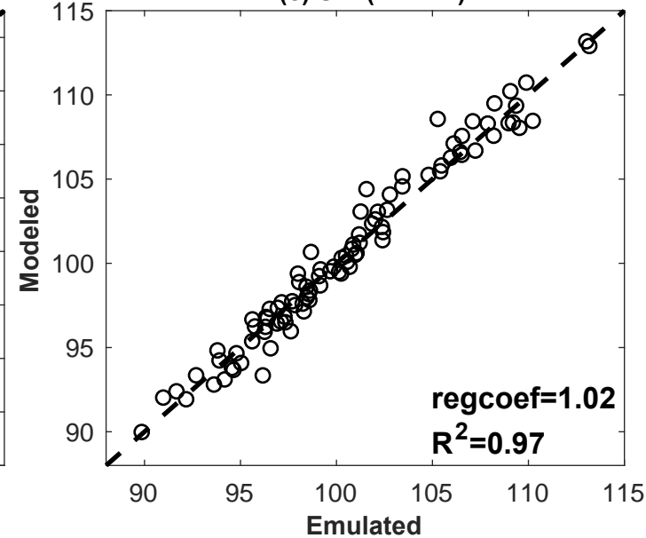
(f) JJAPr bias (%)
