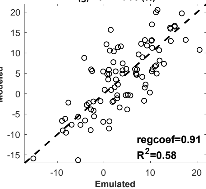
(g) DJFPr bias (%)
