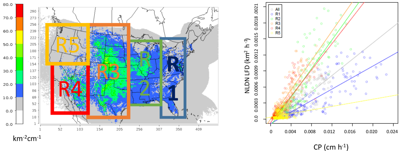
Figure 3. (a) The ratio (background) between lightning flash density and modeled convective precipitation (CP) in July (2002–2014; similar patterns for other months are not shown) and the analysis regions (R1 to R5). (b) Comparison of monthly mean NLDN lightning flash density ( \text{km}^{-2} \text{h}^{-1} ) and modeled convective precipitation for the domain (All) and regions (R1 to R5) from 2002 to 2014. Each plotted pixel represents the monthly mean value: 13 (years) \times 12 (months) total pixels over each region.
