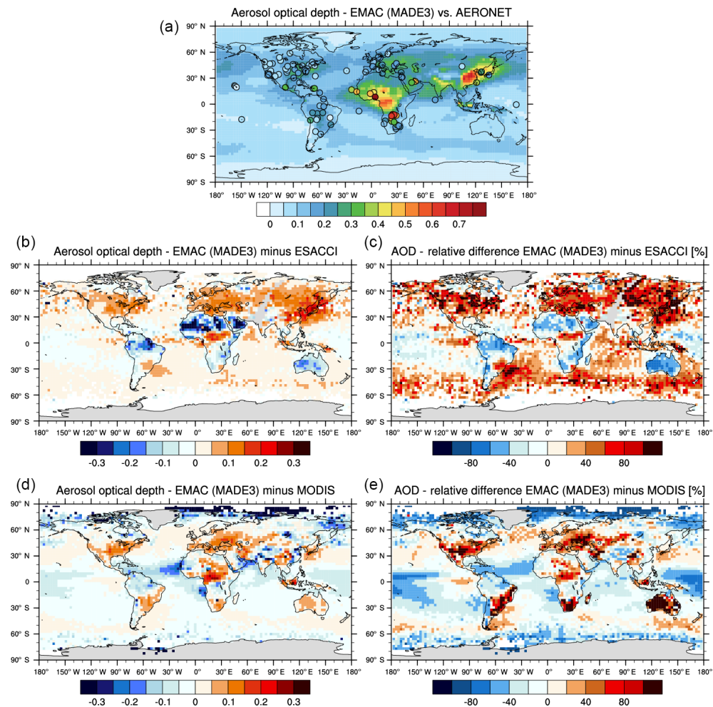
Figure 10. Annual mean AOD in the reference simulation with MADE3 (a, background color) vs. observations from the AERONET network (a, filled circles) and vs. satellite data from the ESACCI Swansea University (SU) ATSR-2 v4.21 aerosol product (b, c) and from MODIS Level 3 Collection 6 (d, e). The comparison against satellite data is shown as both absolute (b, d) and relative (c, e) difference. “Pixels” in the panels correspond to the model grid. Results are shown for the year 2000 (AERONET and ESACCI) and for 2003 (MODIS).
