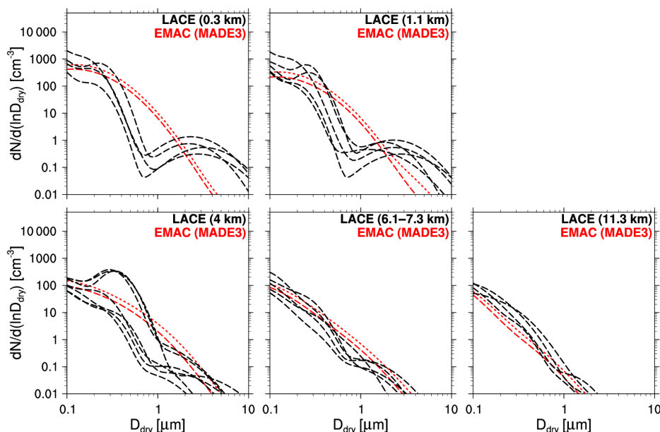
Figure 8. Aerosol particle size distributions in the reference simulation with MADE3 (red) vs. measurements (black) for four to five individual flights (depending on altitude) during the LACE campaign over northeastern Germany. Dashed lines represent mean values; dotted lines represent standard deviations, which are only shown in the direction of larger values for clarity.
