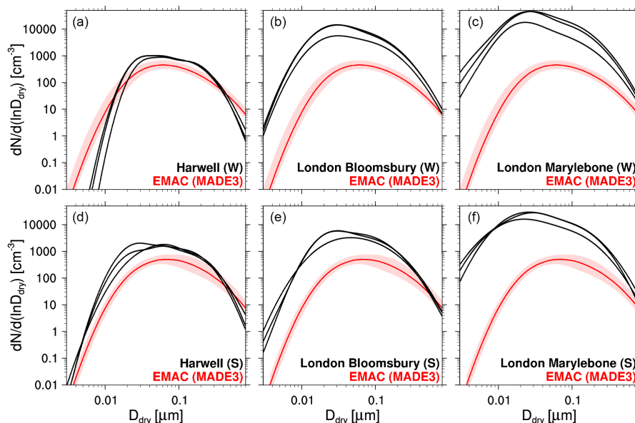
Figure 7. Aerosol particle number size distributions in the EMAC simulation with MADE3 (red) vs. ground-based measurements (Putaud et al., 2003; Van Dingenen et al., 2004) during winter (W, a–c ) and summer (S, d–f ) at the same locations (columns). Each plot contains three measured size distributions: one for the morning, one for the afternoon, and one for the night hours. The three stations represent the following conditions (left to right): rural, urban, and kerb side (terminology adapted from Putaud et al., 2003). All measurement locations fall into the same model grid box, so that the simulated size distribution only differs between the top and bottom rows but not between columns. Solid lines stand for median values; shadings indicate the 25th to 75th percentiles. Note that the vertical axis of the left plot in each row applies to the other plots of that row as well, and the horizontal axes of the plots in the lowermost row also apply to the other plots in the respective columns.
