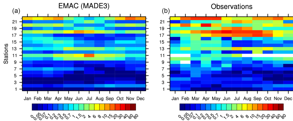
Figure 4. Climatological annual cycle of simulated (a) and measured (b) dust surface-level concentrations in units of \mu\text{g m}^{-3} . The observational data were collected by Huneus et al. (2011). The locations of the 22 stations considered in the plot are shown in Fig. 6 of Aquila et al. (2011).
