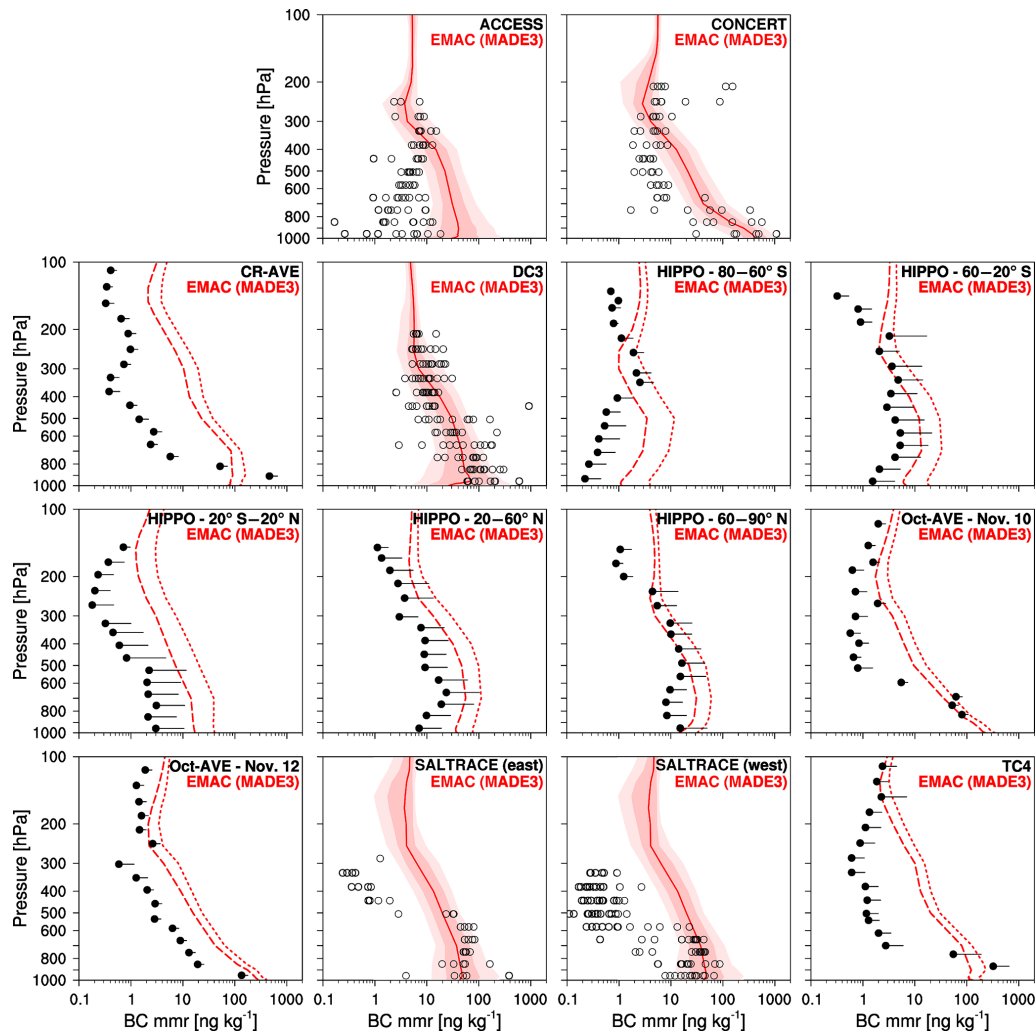
Figure 5. BC mass mixing ratios (mmrs) in the EMAC simulation with MADE3 (red) vs. measurements during various field campaigns (black). Dashed lines and filled circles represent mean values; dotted lines and whiskers represent standard deviations, which are only shown in the direction of larger values for clarity. Solid lines stand for median values. Light and dark shadings indicate the 10th to 90th, and 25th to 75th percentiles, respectively. Hollow circles are the median values of individual flights. Descriptions of the campaigns are provided in Table 4 and in the text. Note that the vertical axis of the left plot in each row applies to the other plots of that row as well, and the horizontal axes of the plots in the lowermost row also apply to the plots in the other rows.
