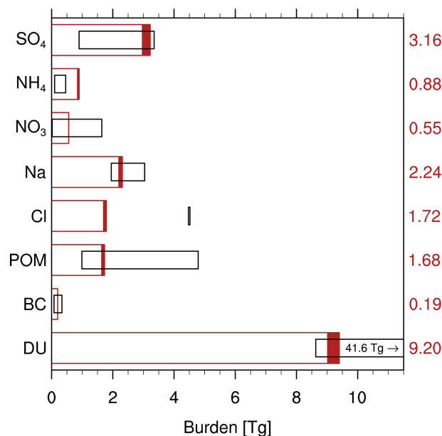
Figure 11. Global tropospheric aerosol burdens simulated by EMAC (MADE3). The filled part of each bar indicates the range of values for the 10 evaluated years. The average values are given on the right side of the plot. The ranges of values from a compilation of other studies (Lauer and Hendricks, 2006; Textor et al., 2006; Bauer et al., 2008; Wang et al., 2009; Mann et al., 2010; Pozzer et al., 2012; Kirkevåg et al., 2013; He and Zhang, 2014; van Noije et al., 2014; Lee et al., 2015; Michou et al., 2015) are shown as black boxes. Values for NH 4 have only been reported by Lauer and Hendricks (2006), Pozzer et al. (2012), and He and Zhang (2014); values for Cl only by He and Zhang (2014). The reported literature range for Na is for sea spray. Note that this is not meant to be a comprehensive literature review but should yield a representative picture. Extreme values may stem from specific sensitivity studies.
