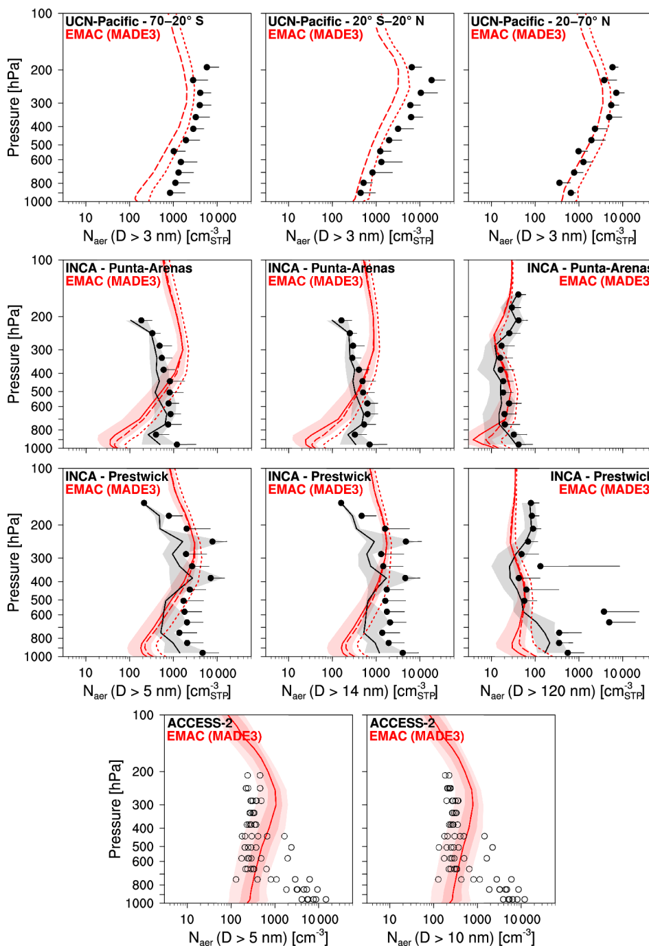
Figure 6. Same as Fig. 5 but for aerosol particle number concentrations with various cutoff diameters.
