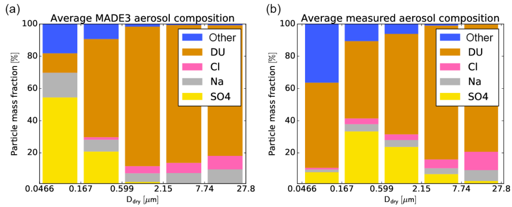
Figure 9. Average size-resolved aerosol composition as simulated by the model (a) and as measured during the SAMUM-2 campaign (b). Only the mass fractions of species that can be compared between measurement data and model output are depicted.
