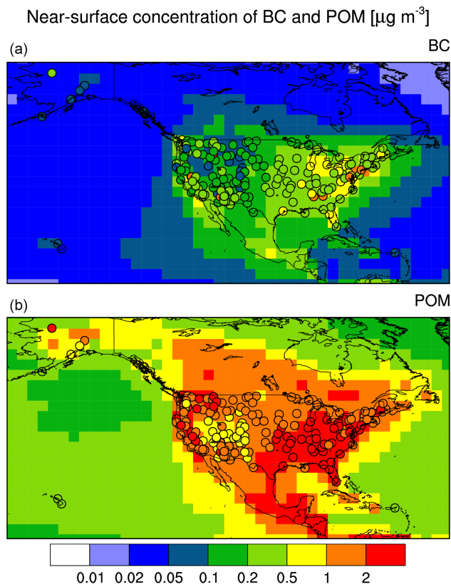
Figure 3. EMAC simulation with MADE3 (background color; “pixels” correspond to the model grid) vs. observations from the station network IMPROVE (filled circles): near-surface BC (a) and POM (b) mass concentrations.
