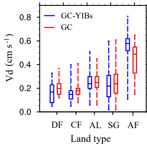
(f) Dry deposition velocity
