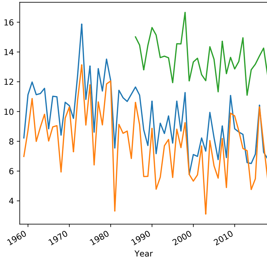
(b) Abyssal overturning at 40°S
