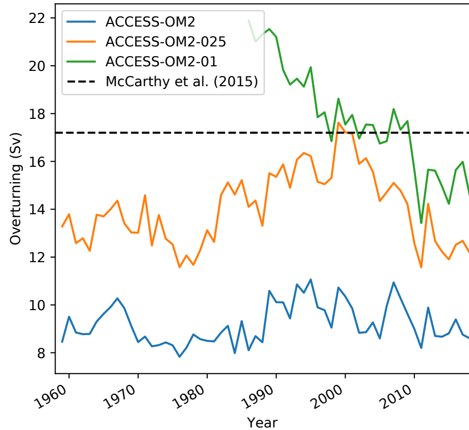
(a) AMOC at 26°N
